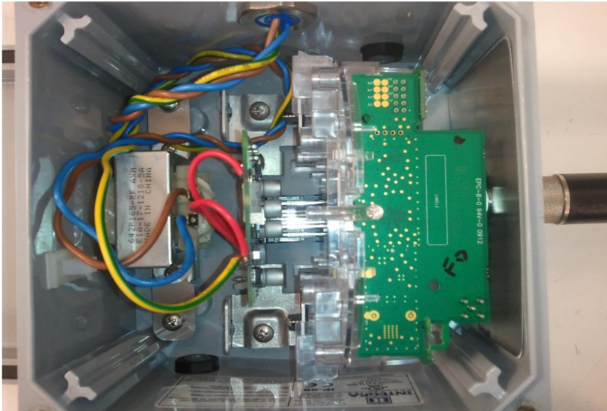
Figure 1 Itron AMI7 module, FCC ID: SK9AMI7, IC: 864G-AMI7
