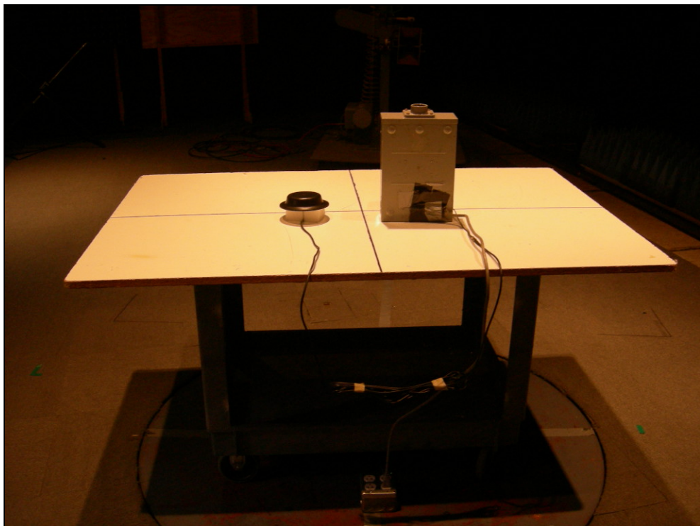
Figure 2: Radiated Emissions - Low Profile Radome Antenna
