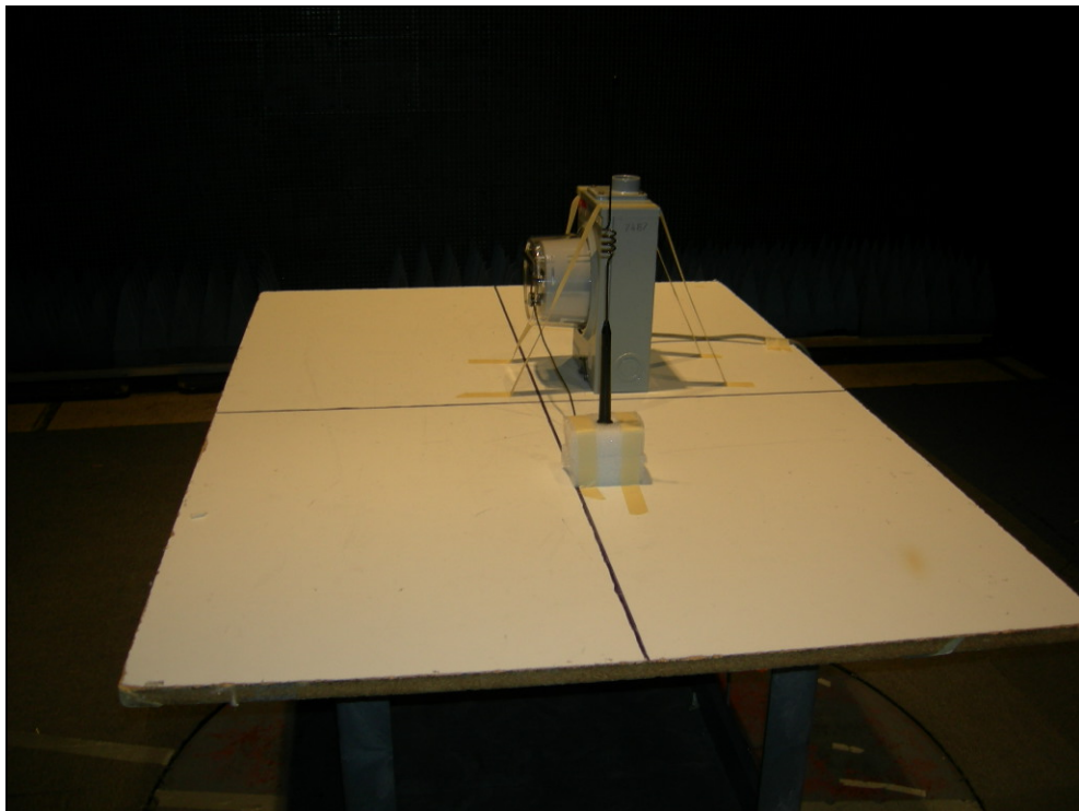
Figure 8: Radiated Emissions – Whip Antenna
