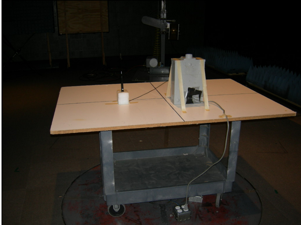
Figure 6: Radiated Emissions – Whip Antenna
