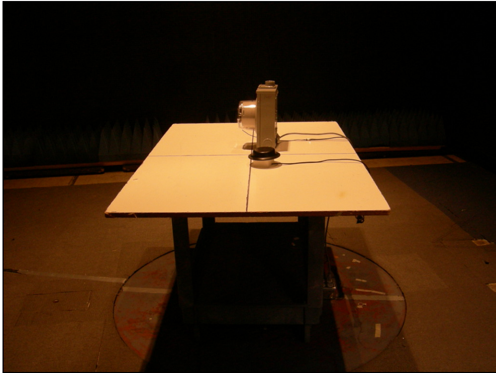
Figure 3: Radiated Emissions – Low Profile Radome Antenna
