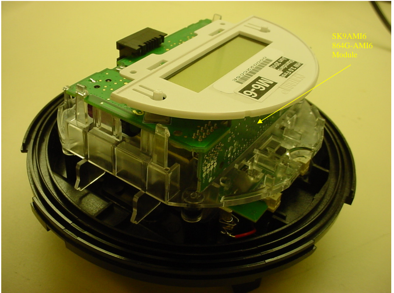
Figure 1: Module Location – 3S Meter
