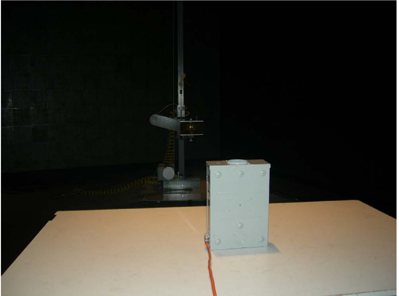
Figure 1: Radiated Emissions, 3S Meter
