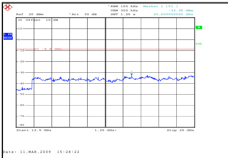
Figure 7.6.2.2-9: 12.5 GHz – 25 GHz –High Channel
