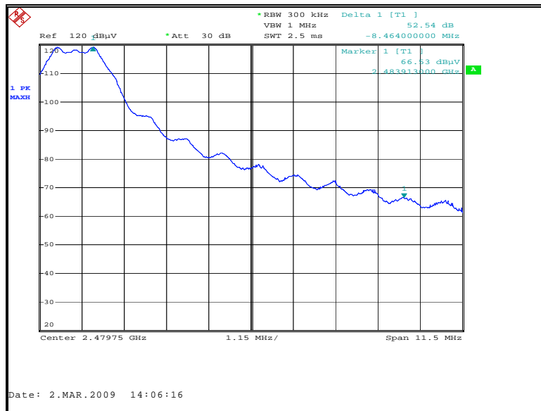
Figure 7.6.1.2-1: Upper Band-edge (Radiated) – 3S
