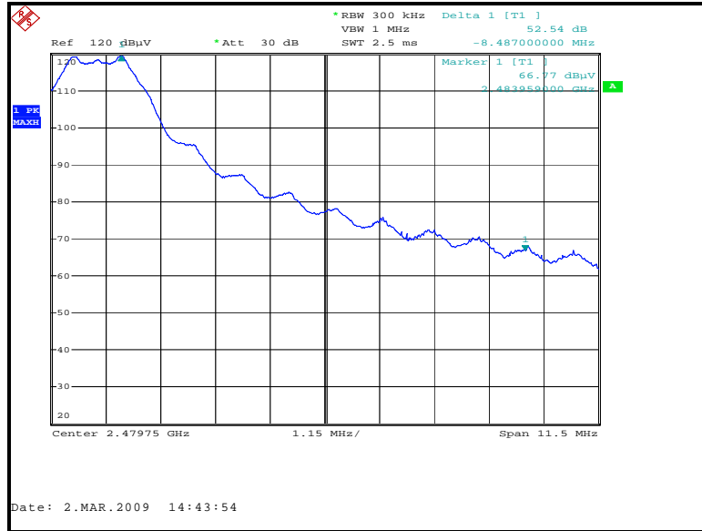
Figure 7.6.1.2-2: Upper Band-edge (Radiated) – 4S
