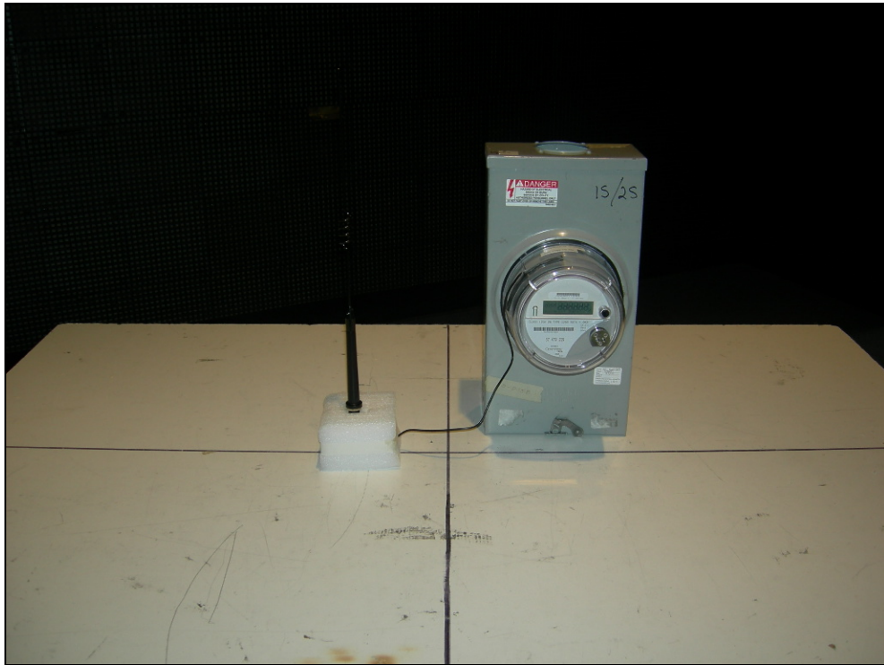
Figure 1: Radiated Emissions – Whip Antenna
