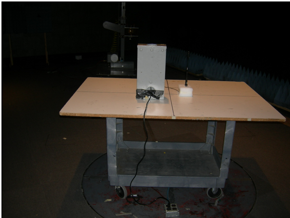
Figure 2: Radiated Emissions – Whip Antenna
