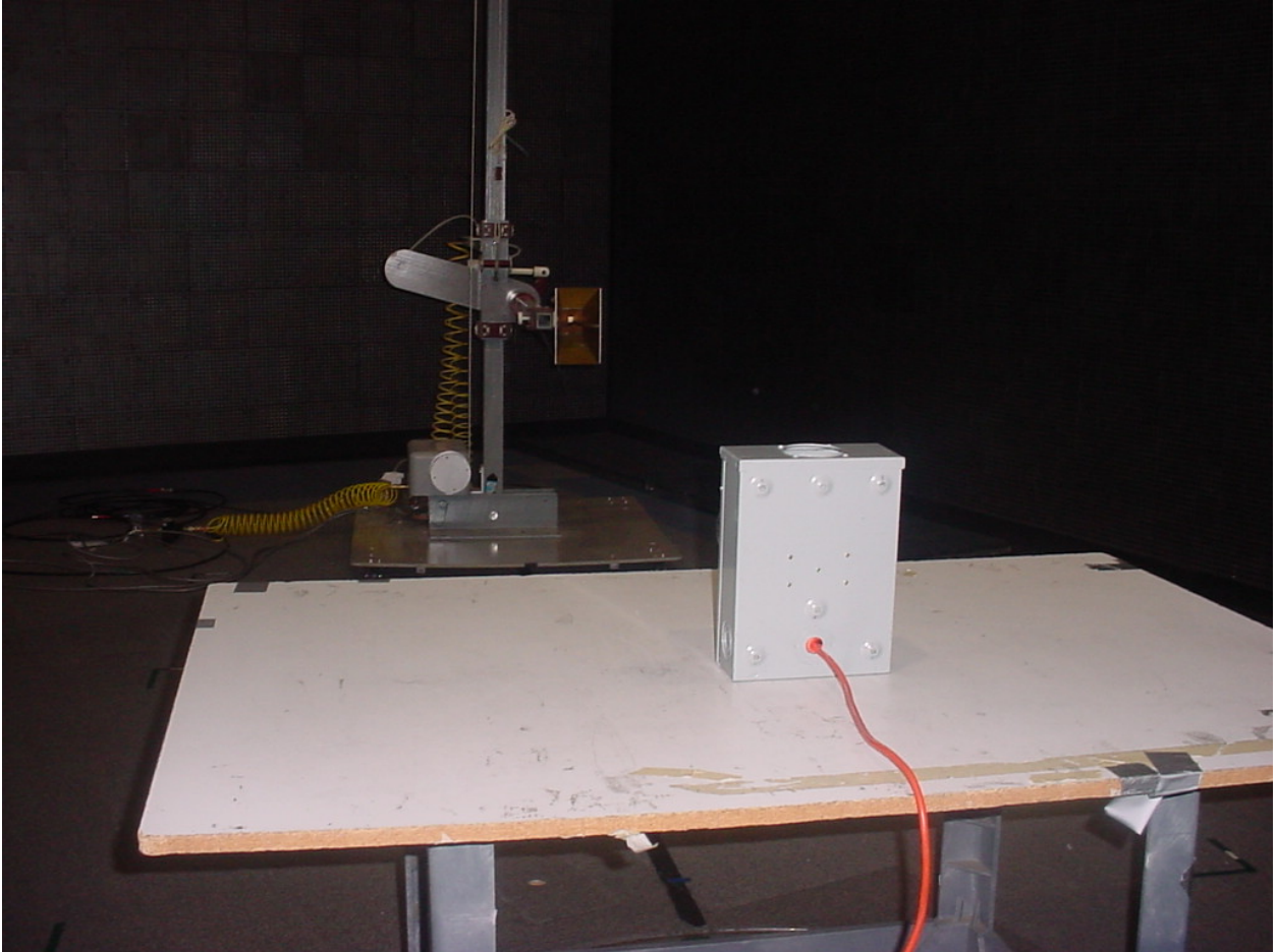
Figure 6: Radiated Emissions – CVSOD-A
