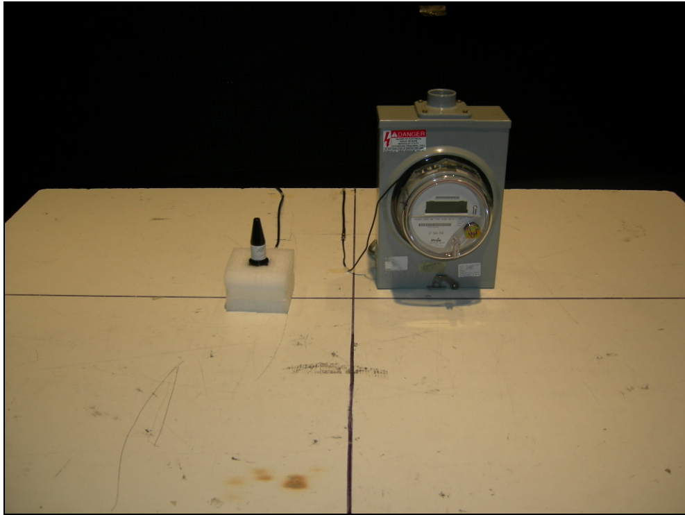
Figure 3: Radiated Emissions – Stub Antenna
