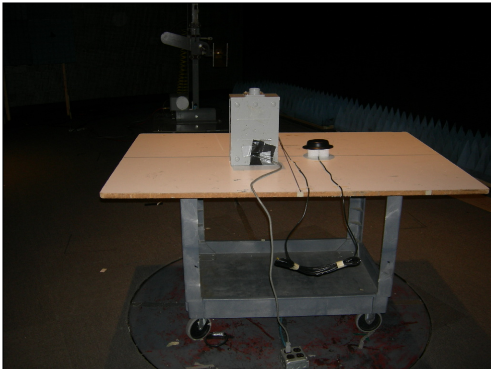
Figure 2: Radiated Emissions – Radome Antenna
