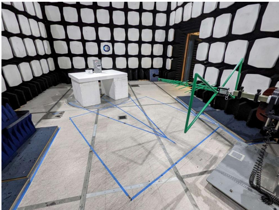
Figure 6: Equipment Under Test – Radiated Emissions <1GHz-Radme Antenna
