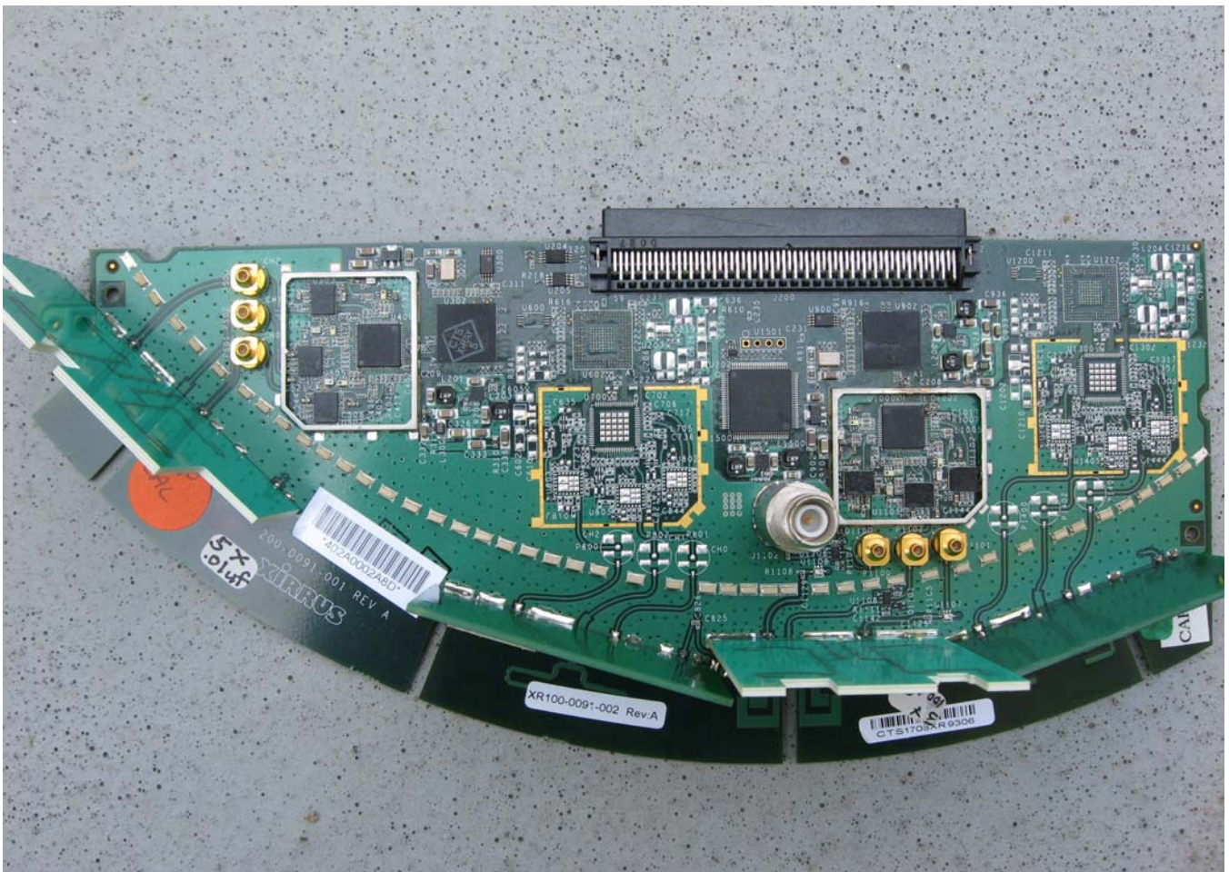
RF board - two transceivers per board (2 depopulated)
