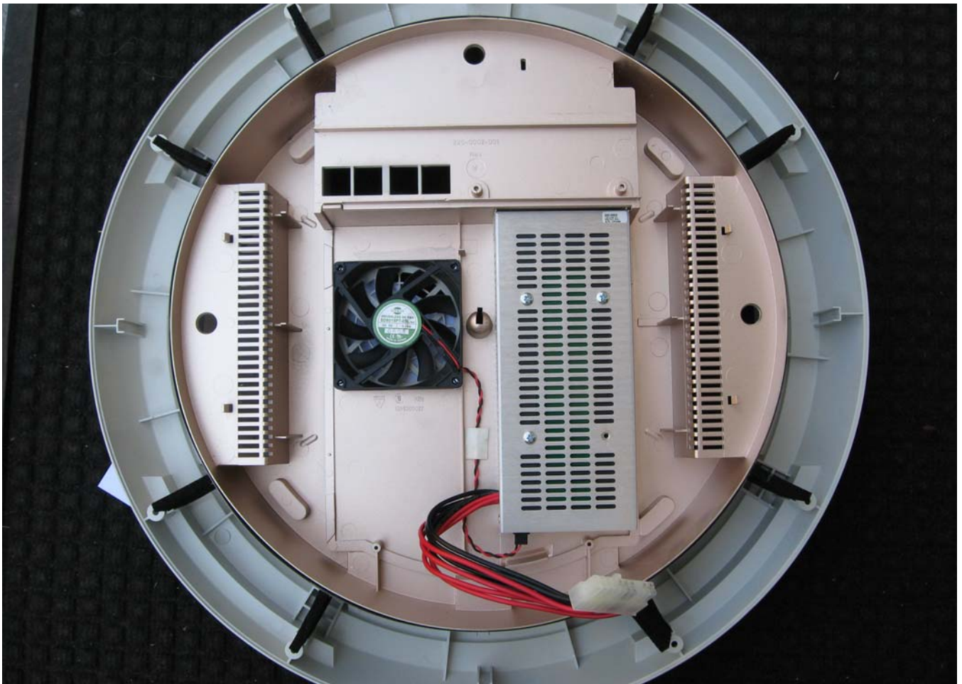
Internal view - base below and top above
