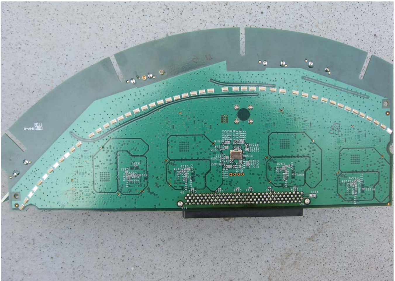
RF board - two transceivers per board (2 depopulated)
