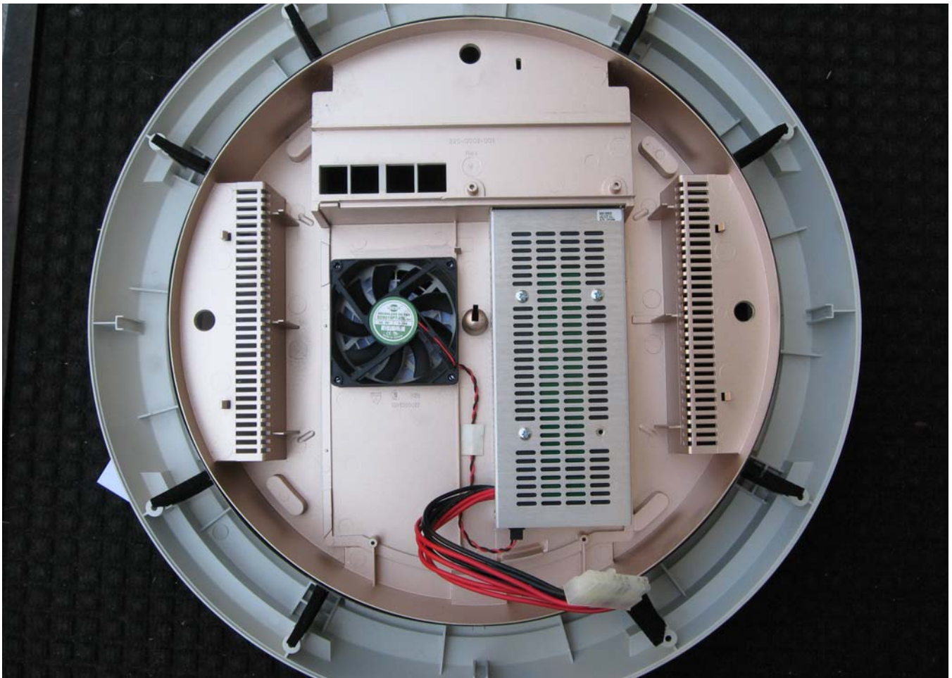
Internal view of enclosure - top (above) and base (below)
