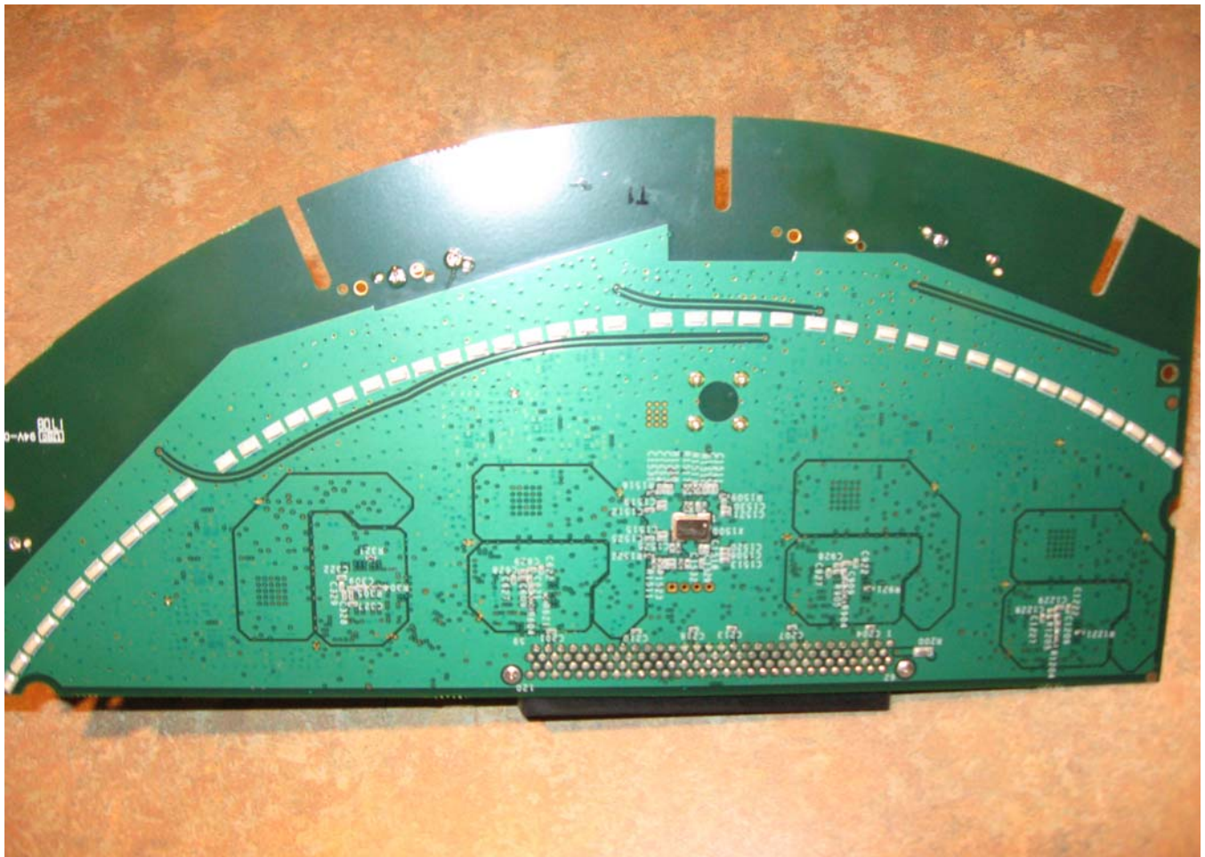
RF Board with 4 transceivers per board - top and bottom
