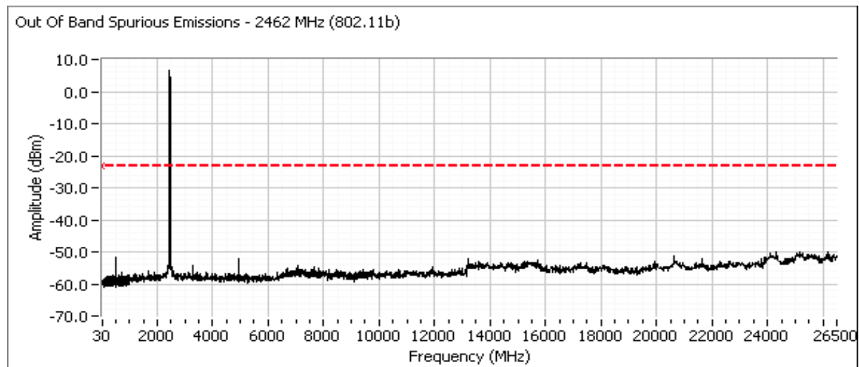
Plots for high channel - 802.11b - , power setting(s) = 18.5
