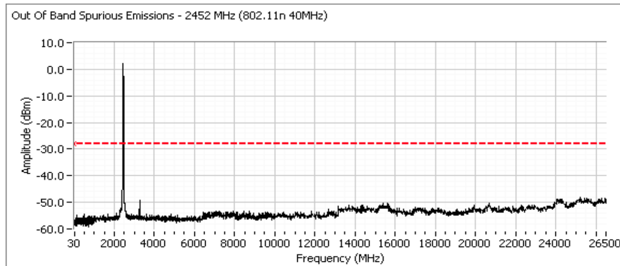
Plots for high channel - 802.11n40 - , power setting(s) = 9.0
