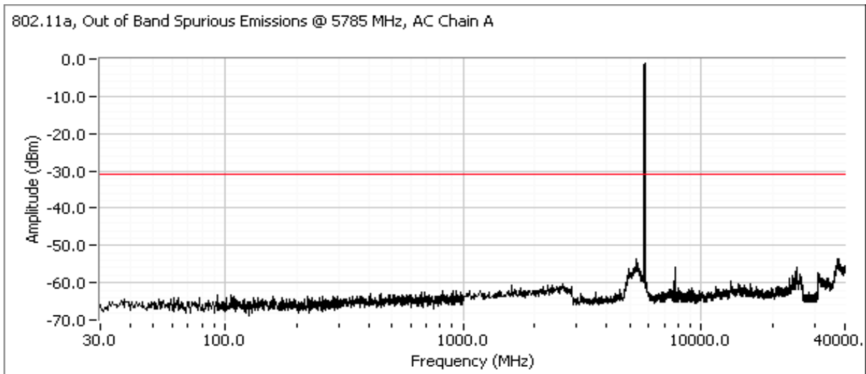
Plots for center channel - 802.11a - , power setting(s) = 17
