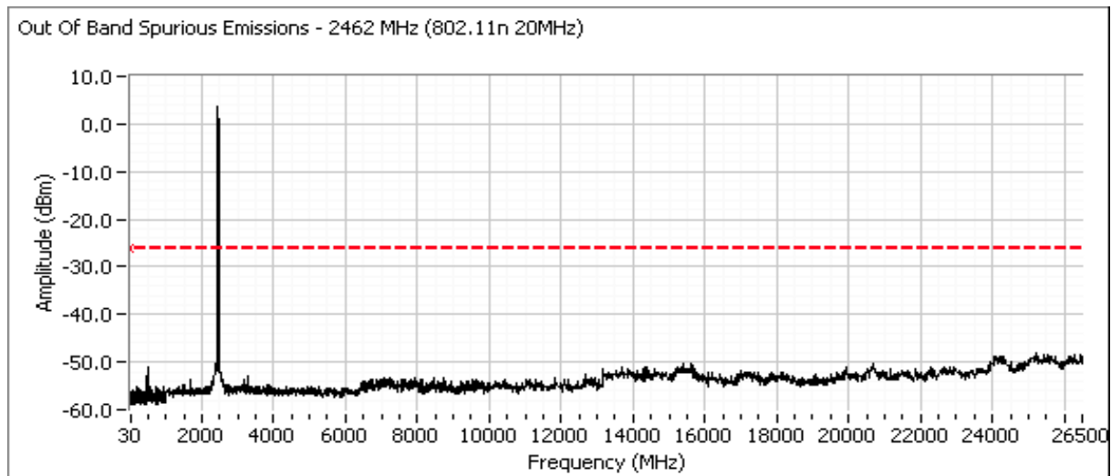
Plots for high channel - 802.11n20 - , power setting(s) = 9.5
