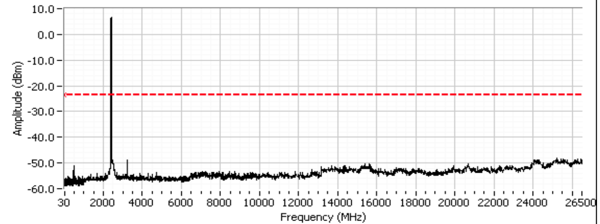
Out Of Band Spurious Emissions - 2412 MHz (802.11n 20MHz)
