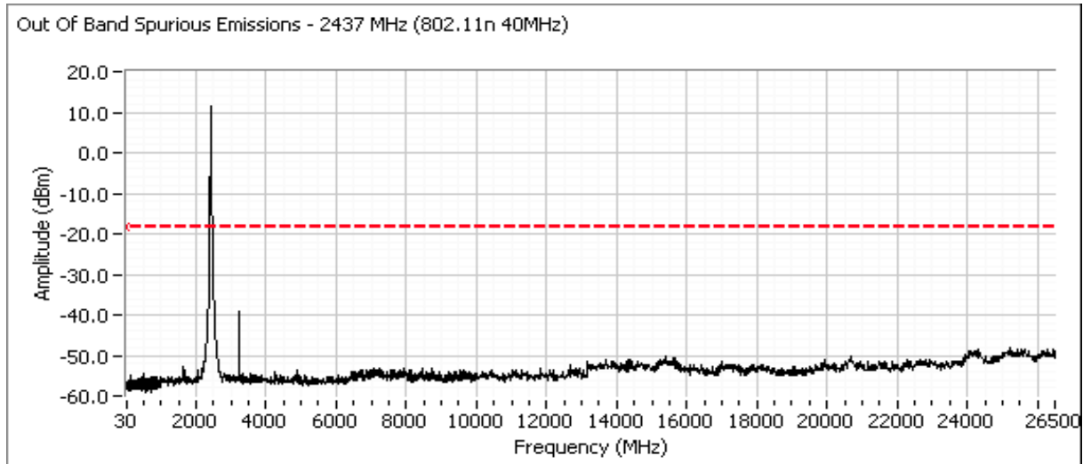
Plots for center channel - 802.11n40 - , power setting(s) = 20.0
