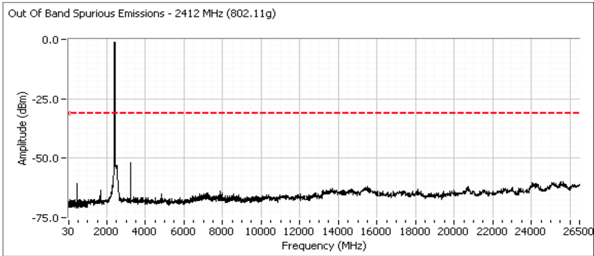
Plots for low channel - 802.11g - , power setting(s) = 13.5
