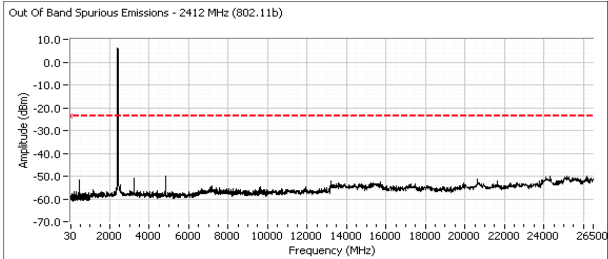
Out Of Band Spurious Emissions - 2412 MHz (802.11b)
