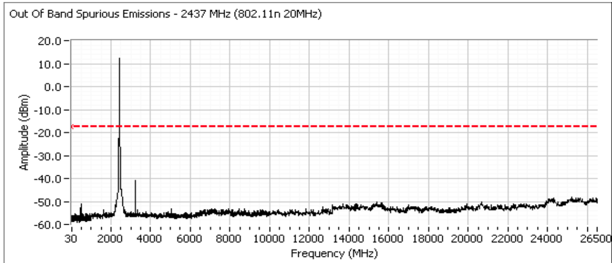
Plots for center channel - 802.11n20 - , power setting(s) = 20.0
