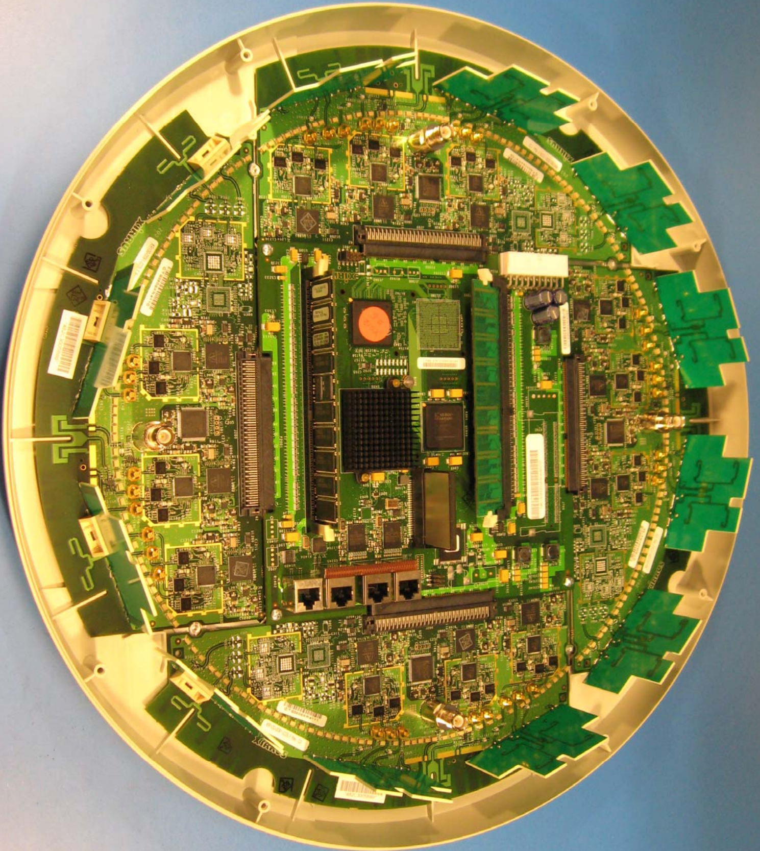
Internal View - Radio Boards and Main Digital Board
