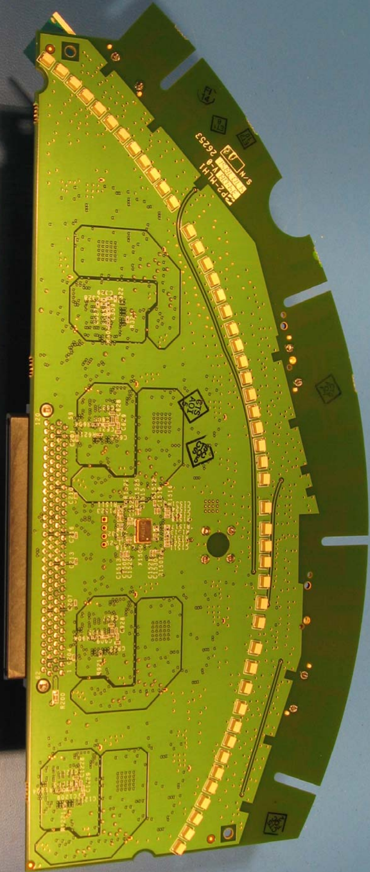
Radio Board (3 Transceivers installed for XN12) Bottom View
