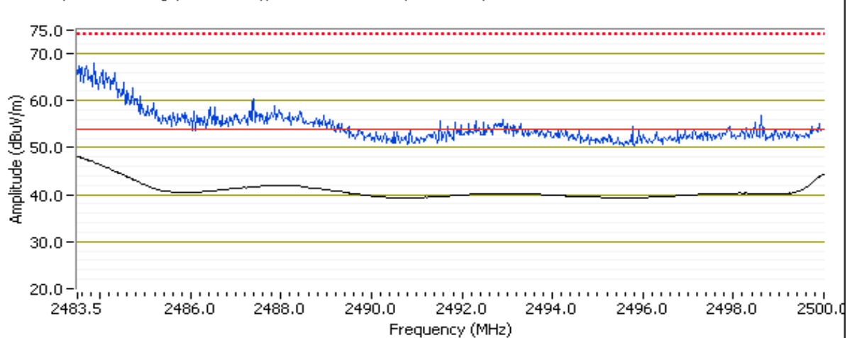
RB 1 MHz; VB 10 Hz Avg (Black Trace), RB=VB=1MHz Pk (Blue Trace) Vertical
