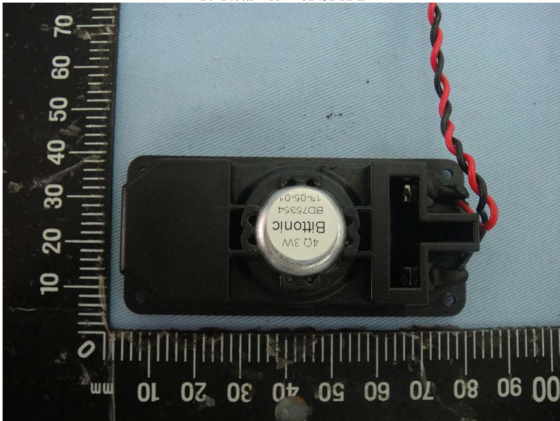
17 Rear view of SPK 2
