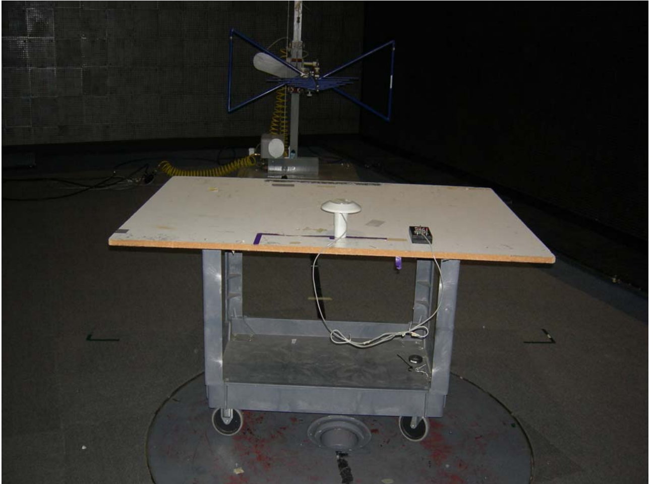
Figure 5: Unintentional Radiated Emissions – Pit Unit
