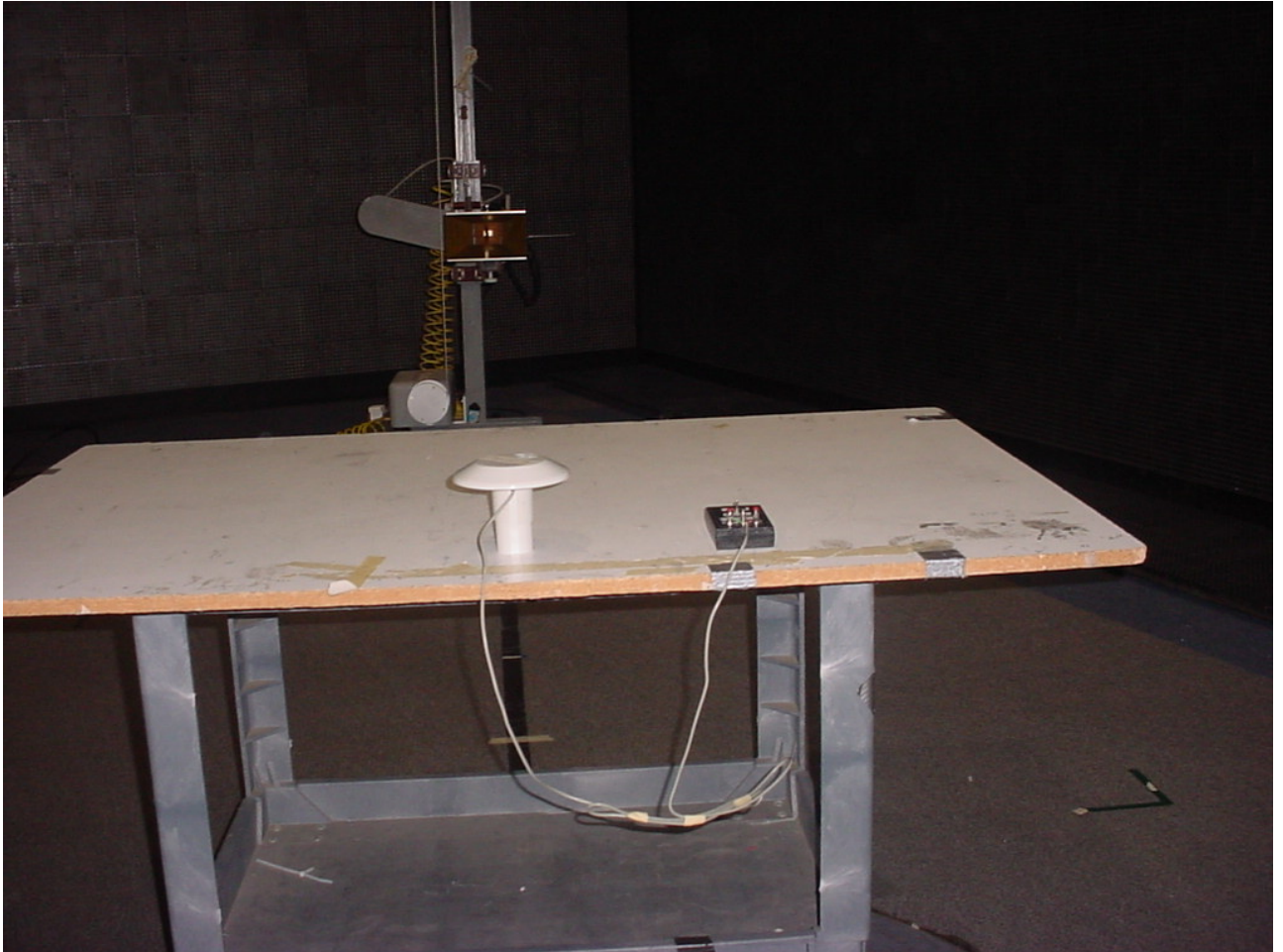
Figure 2: Intentional Radiated Emissions – Pit Unit
