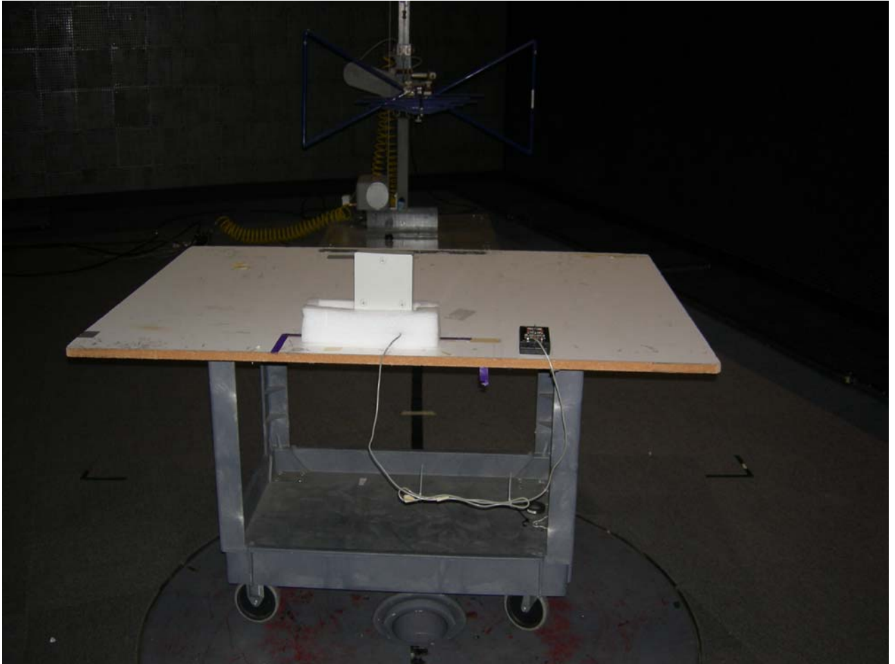
Figure 7: Unintentional Radiated Emissions – Wall Unit
