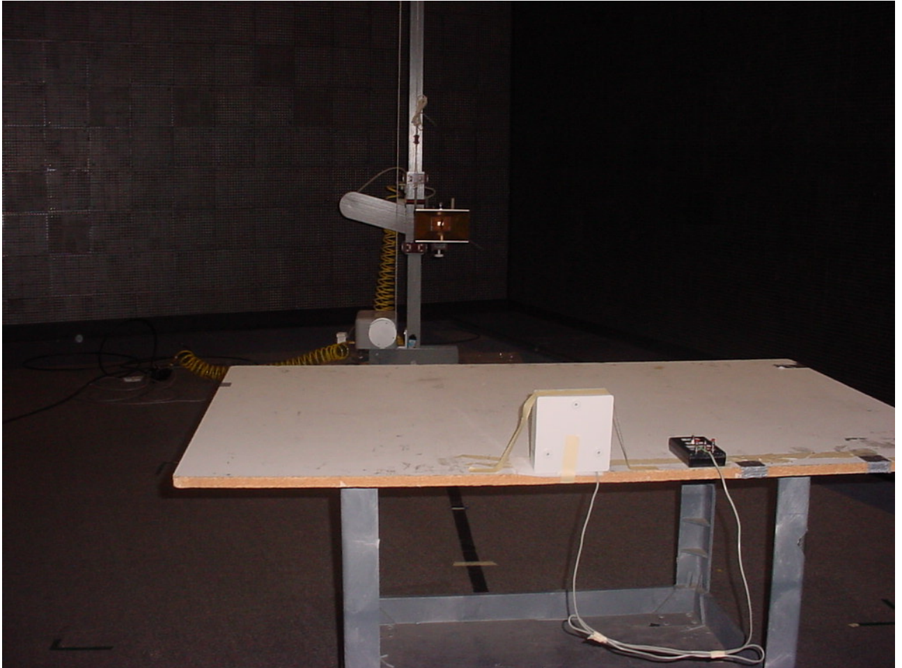
Figure 3: Intentional Radiated Emissions – Wall Unit
