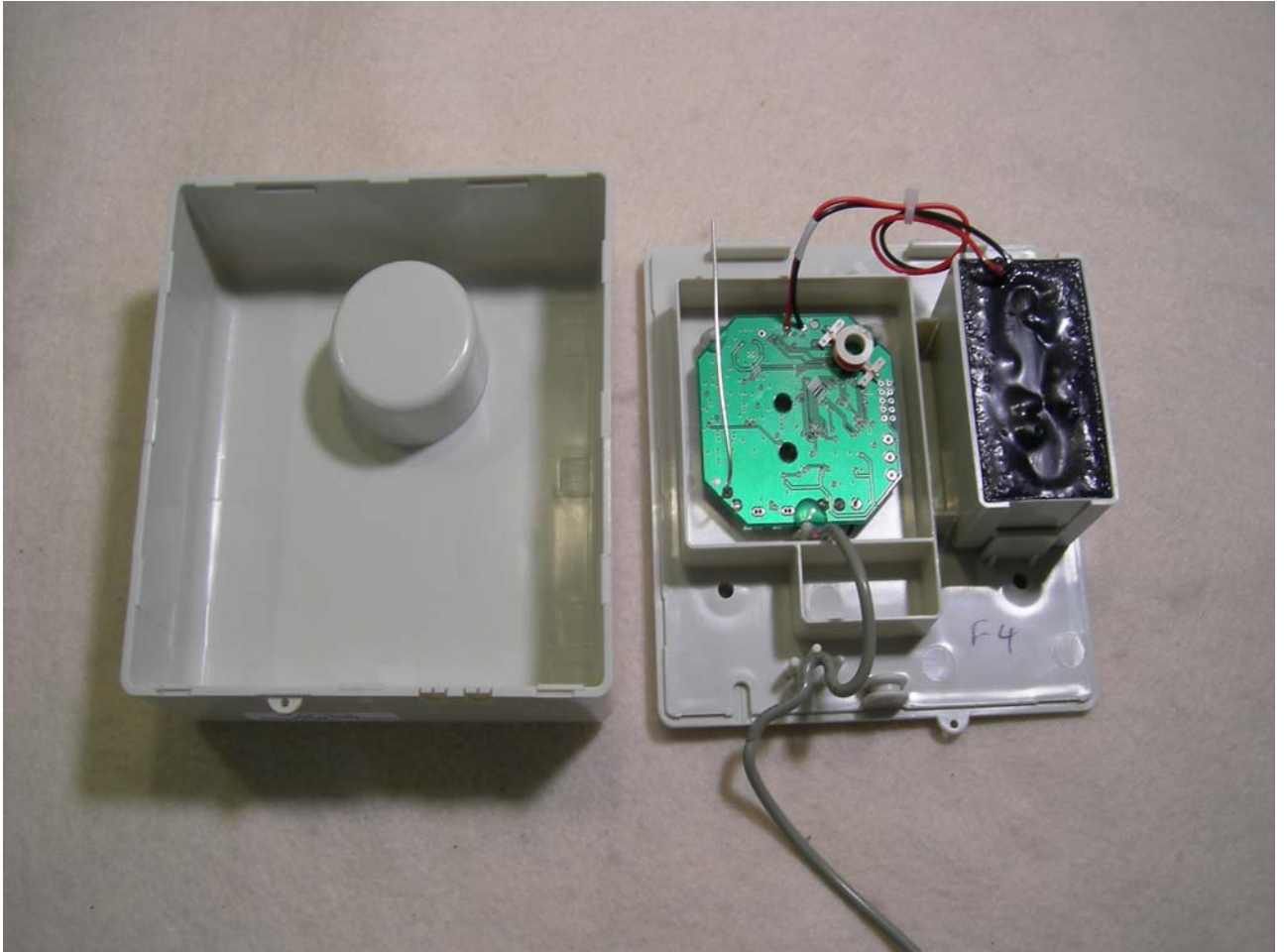
Figure 1: Wall Mount – PCB Internal Overview
