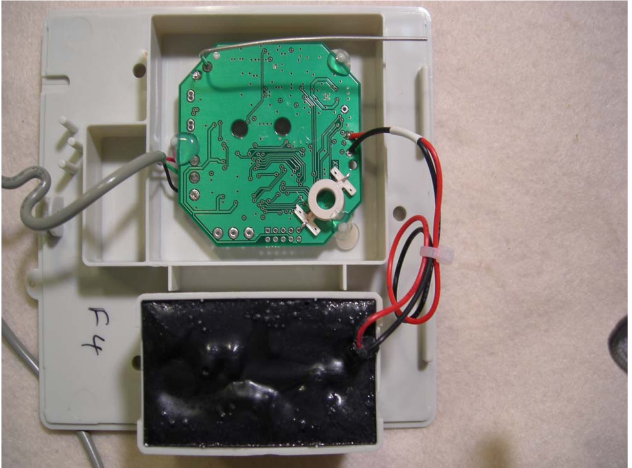
Figure 2: Wall Mount – Battery Location
