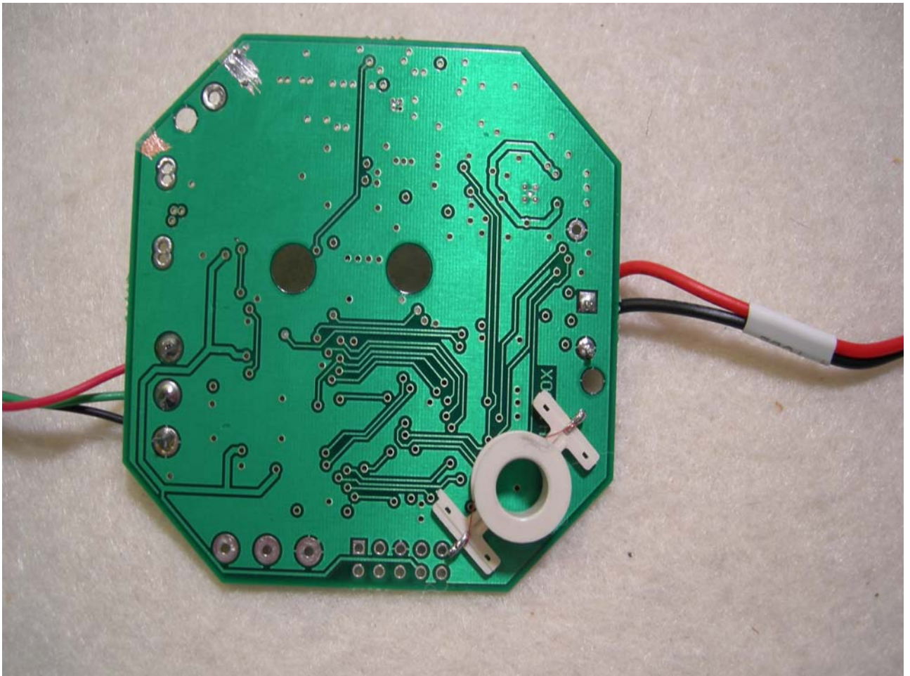
Figure 7: PCB – Bottom View
