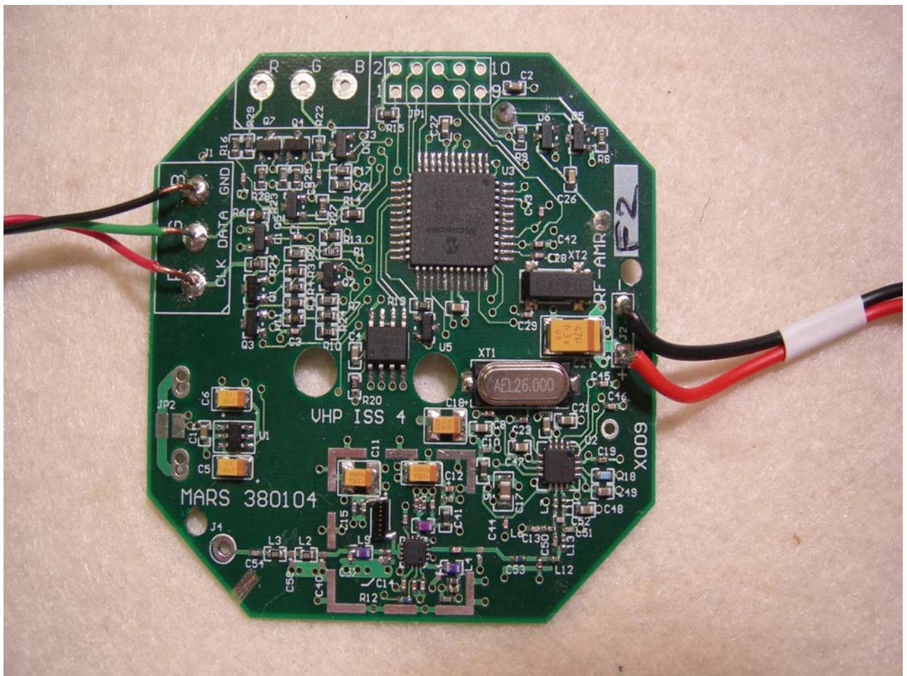
Figure 6: PCB– Top View
