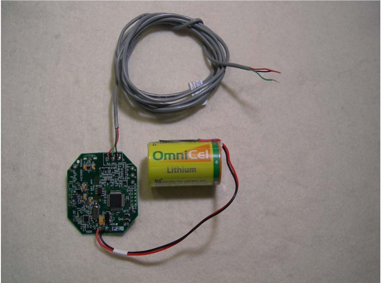
Figure 5: PCB with Battery Attached
