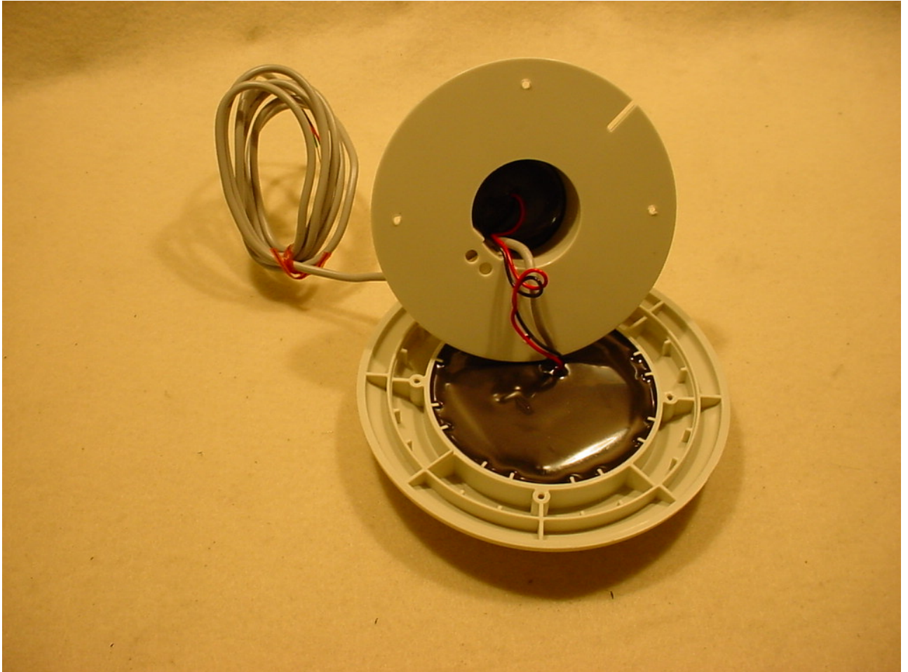
Figure 1: Internal – In Case With Battery
