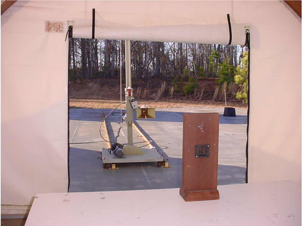
Figure 3: Test Setup Radiated Emissions - Intentional
