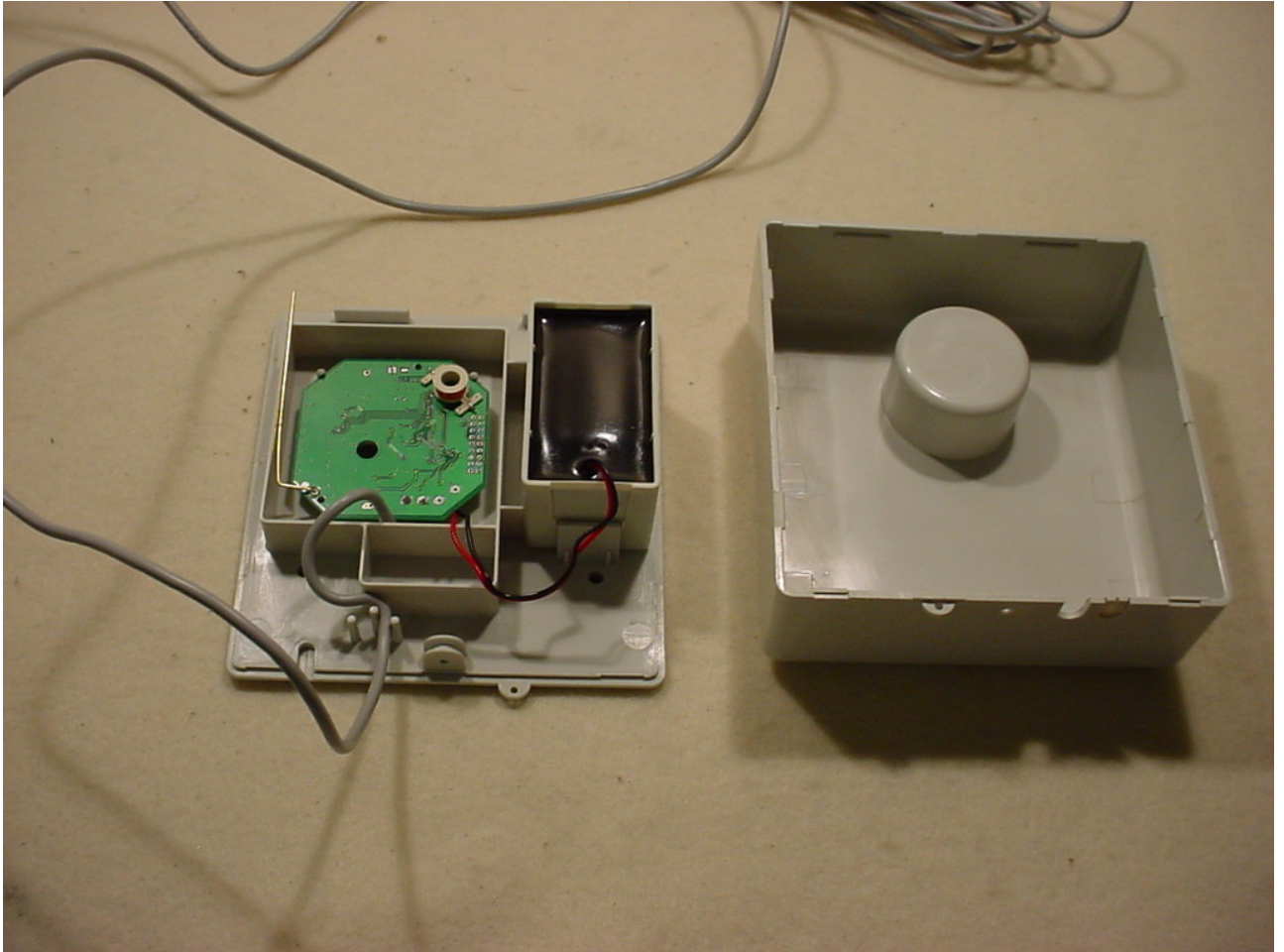
Figure 1: Internal – In Case With Battery
