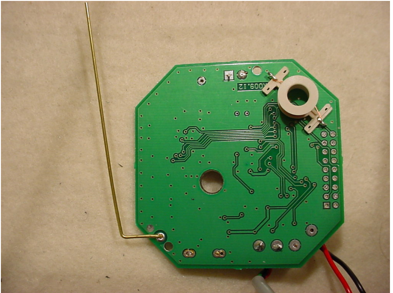
Figure 3: Internal – Back View
