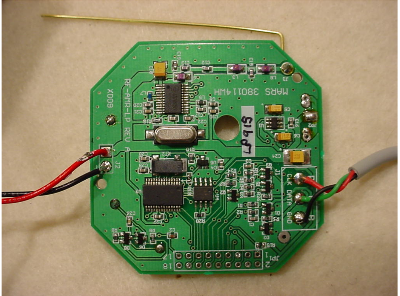
Figure 2: Internal – Front View
