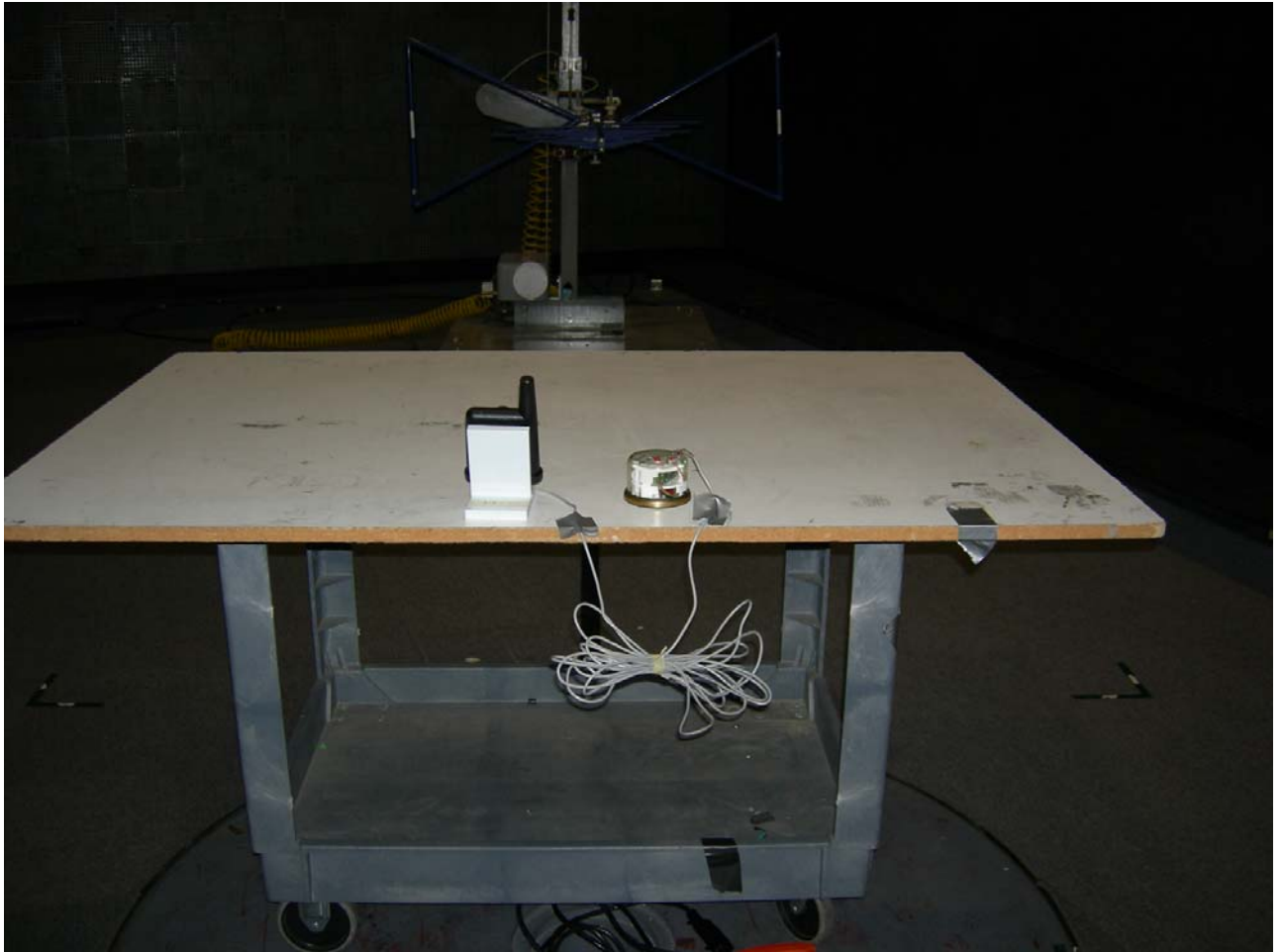
Figure 1: Test Setup Radiated Emissions - Unintentional
