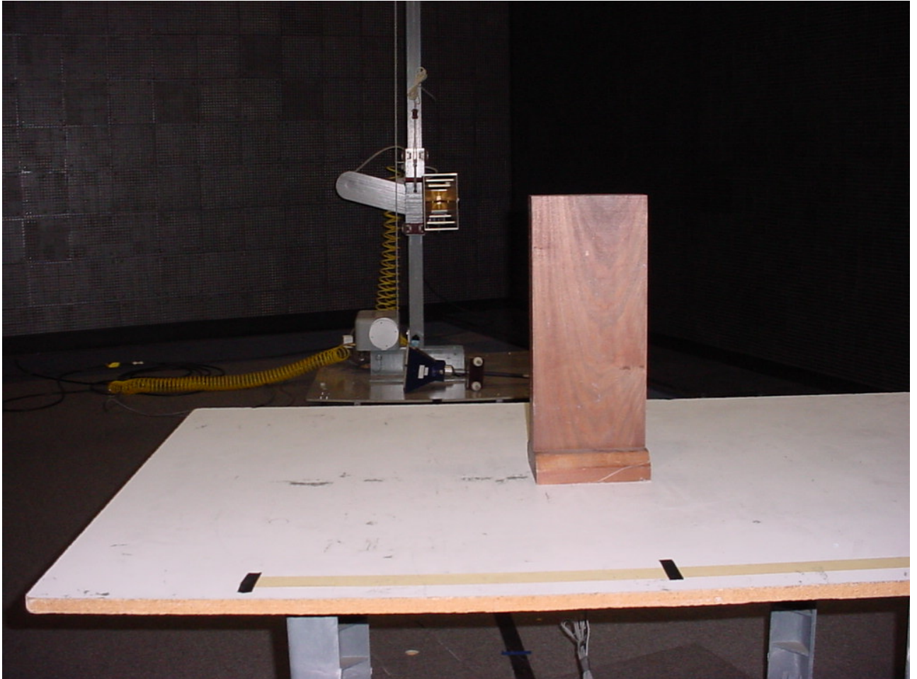
Figure 7: Test Setup Radiated Emissions - Intentional
