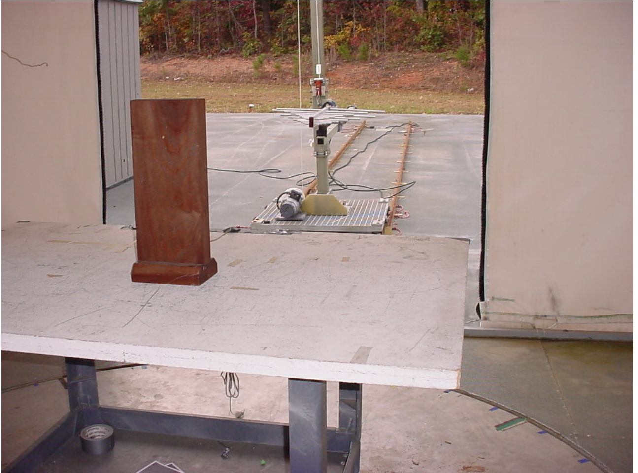
Figure 4: Test Setup Radiated Emissions - Intentional
