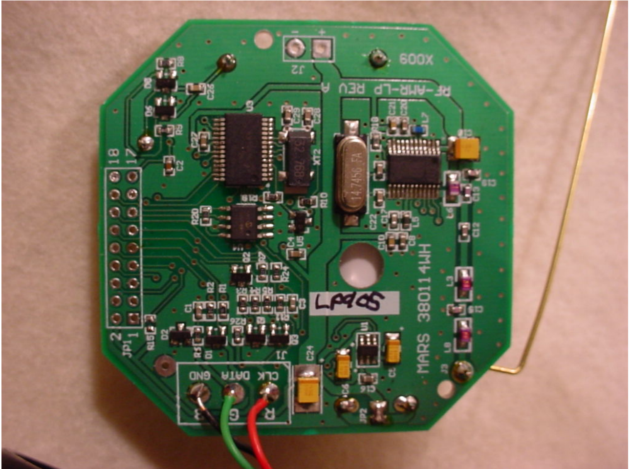
Figure 1: Internal – Front View
