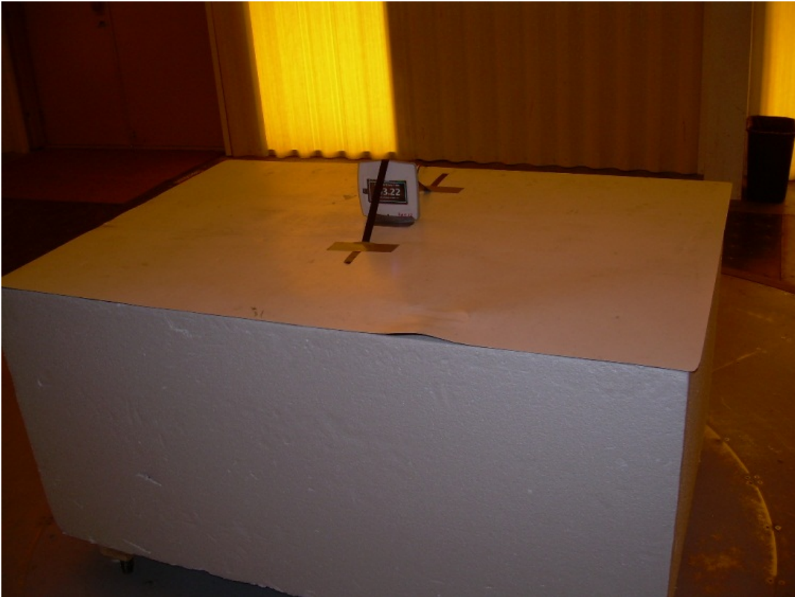
Front View Radiated Disturbance Worst Case Configuration
