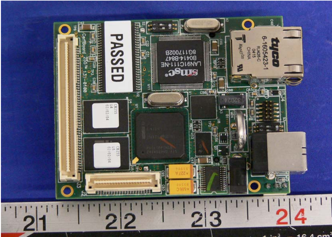
Top Board Solder View
