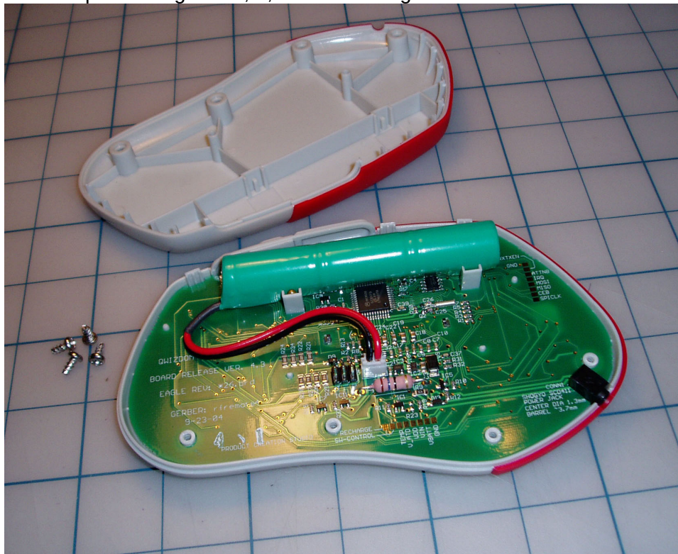
Fig 6 – Q5 RF circuit board in housing.
