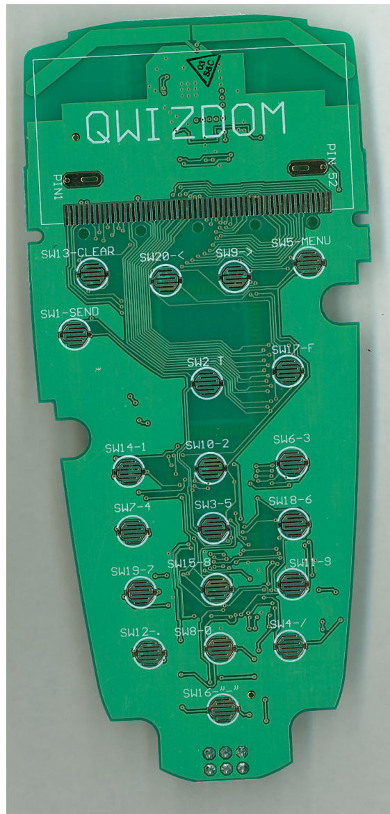
Fig 8 – Bottom Side of Q4 RF circuit board.
