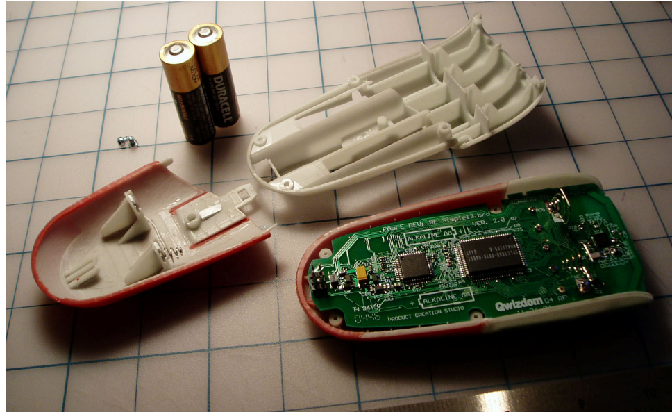
Fig 6 – Q4 RF circuit board in housing.
