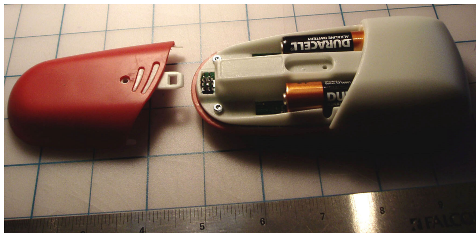
Fig 4 – Back and Battery cover of Q4 RF
