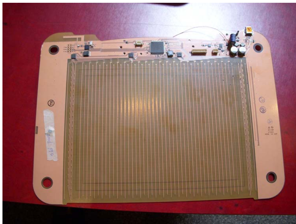
Fig 6 – Q Host PCB side 2.
