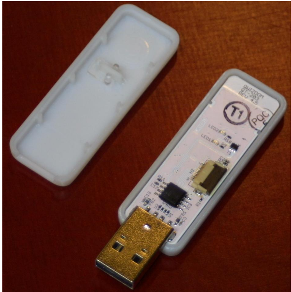
Fig 5 – Q Host circuit board in housing. PCB side 1.
