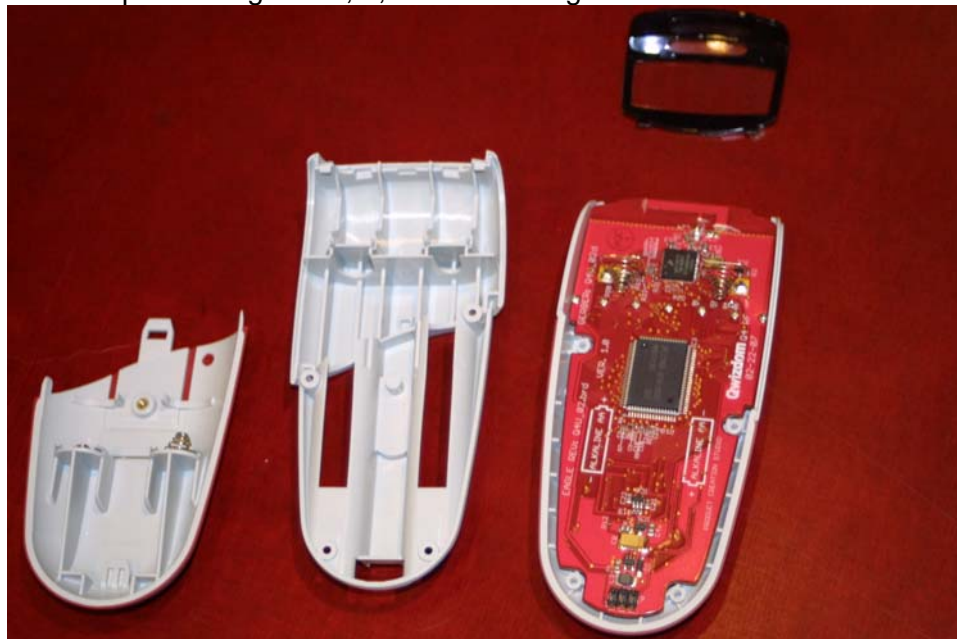
Fig 6 – Q4 RF circuit board in housing.
