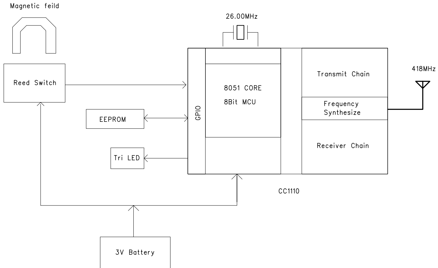
Figure 1. XWS15D-S Diagram block
