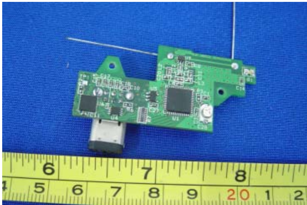
PCB - Component View
