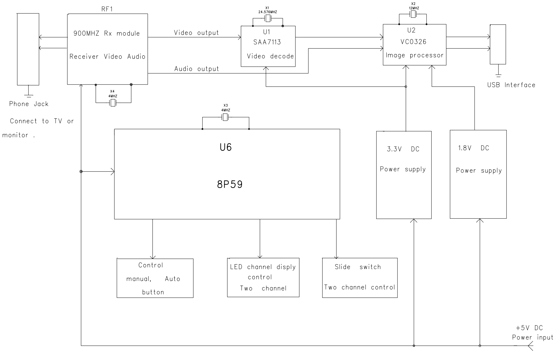
Figure1. Rx230 USB wireless receiver block
