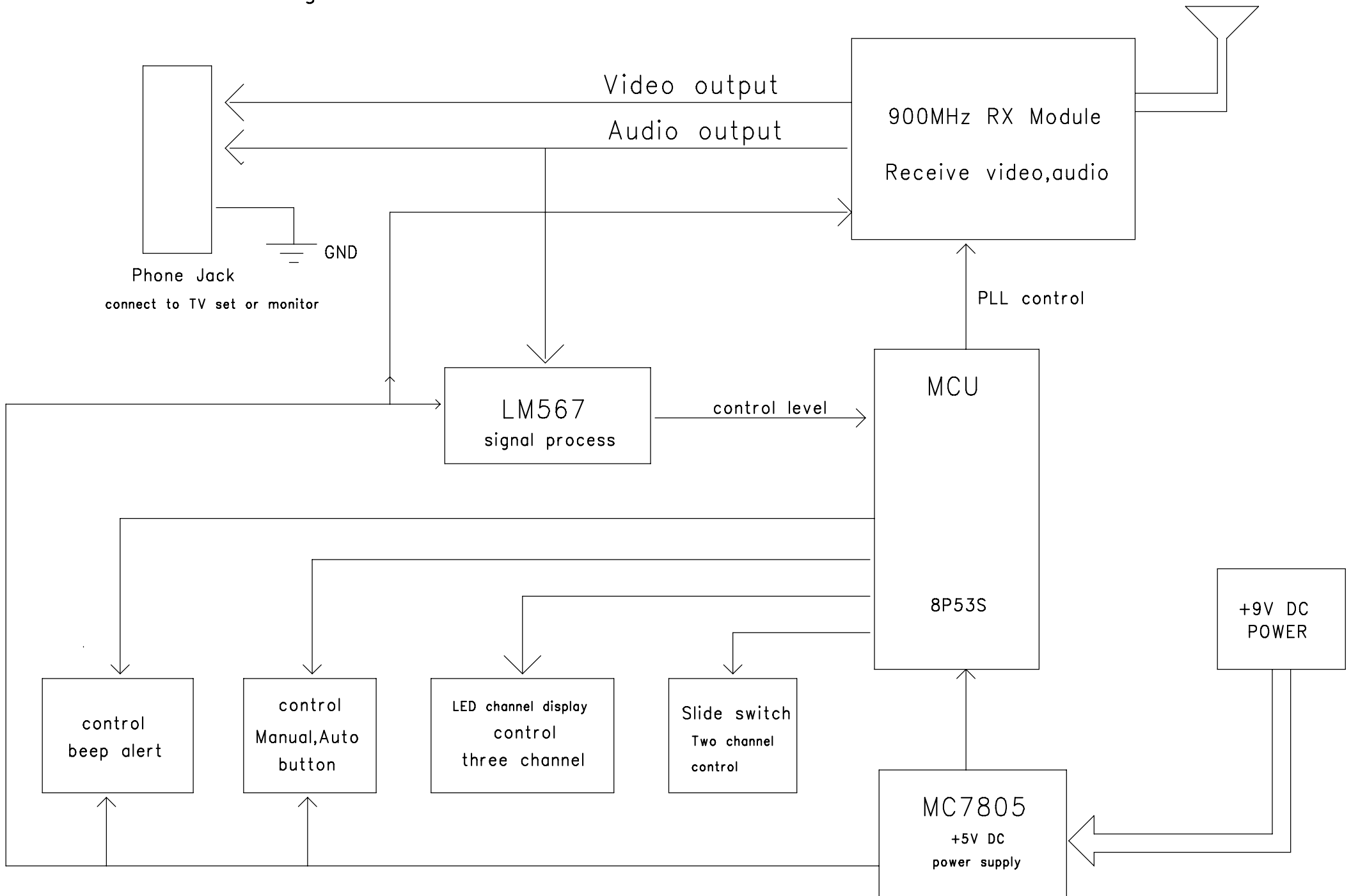
Figure 1. RX200 wireless receiver block
