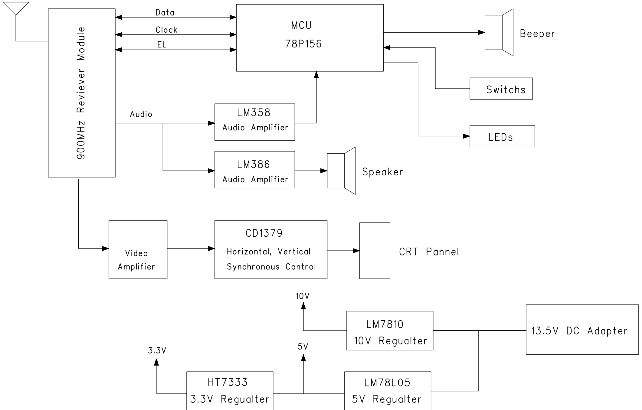
Figure 1. M550 Block Diagram
