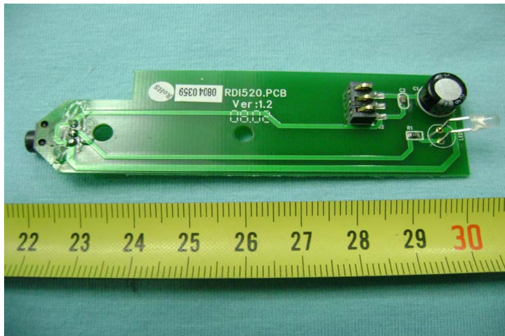
PCB of Battery Charging Base - Front View
