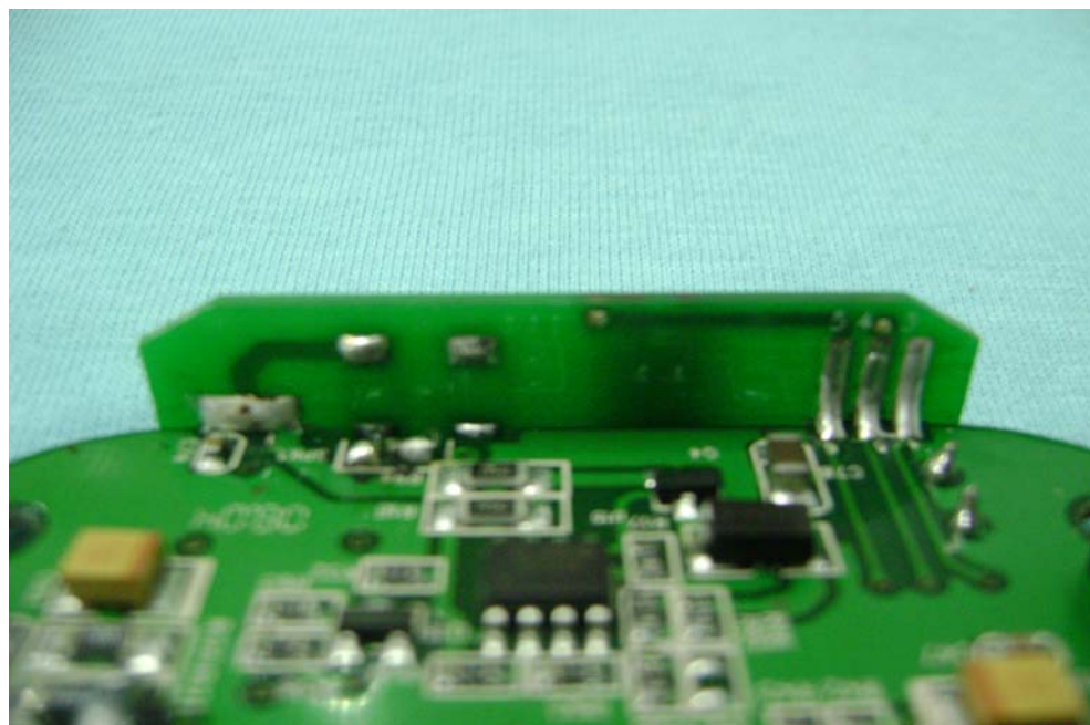
PCB3 of Monitor - Back View
