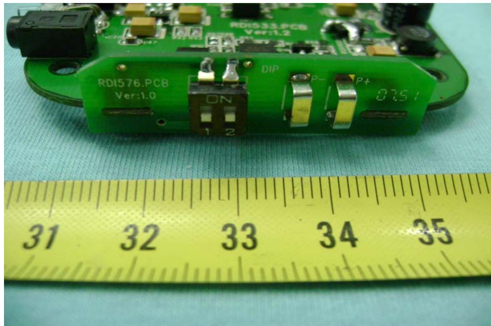
PCB3 of Monitor - Front View
