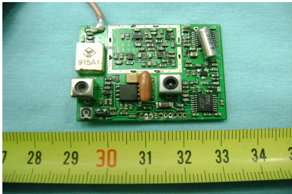
PCB1 of Monitor - Front View
