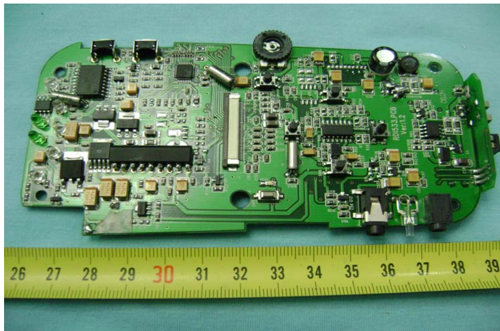
PCB2 of Monitor - Front View
