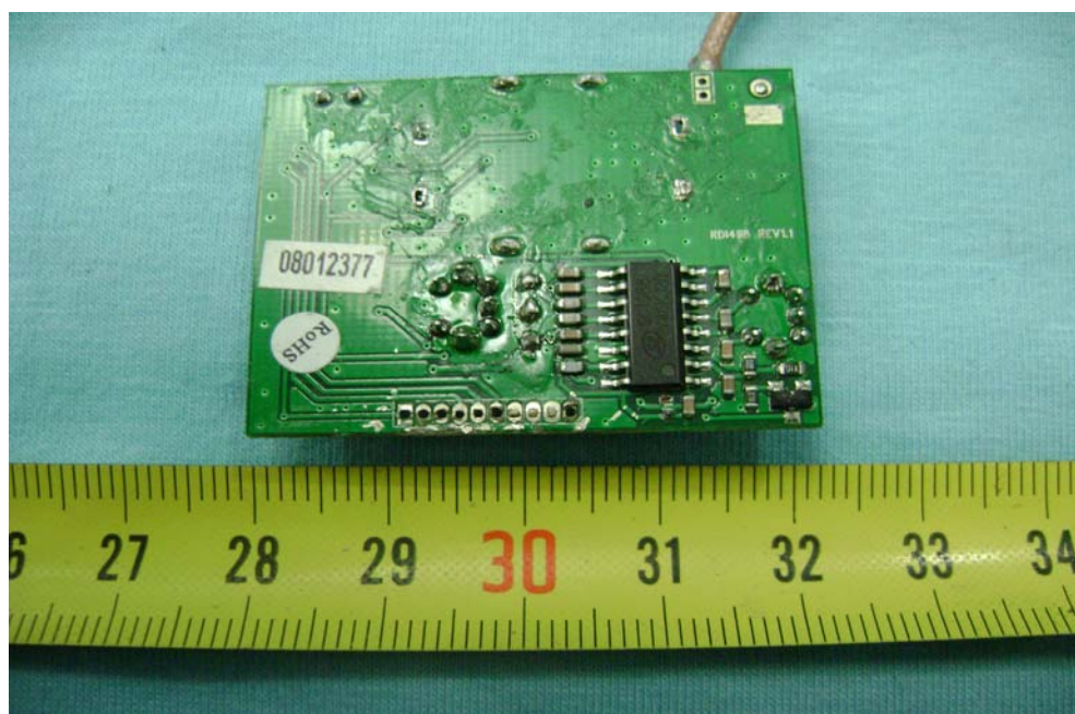
PCB1 of Monitor - Back View
