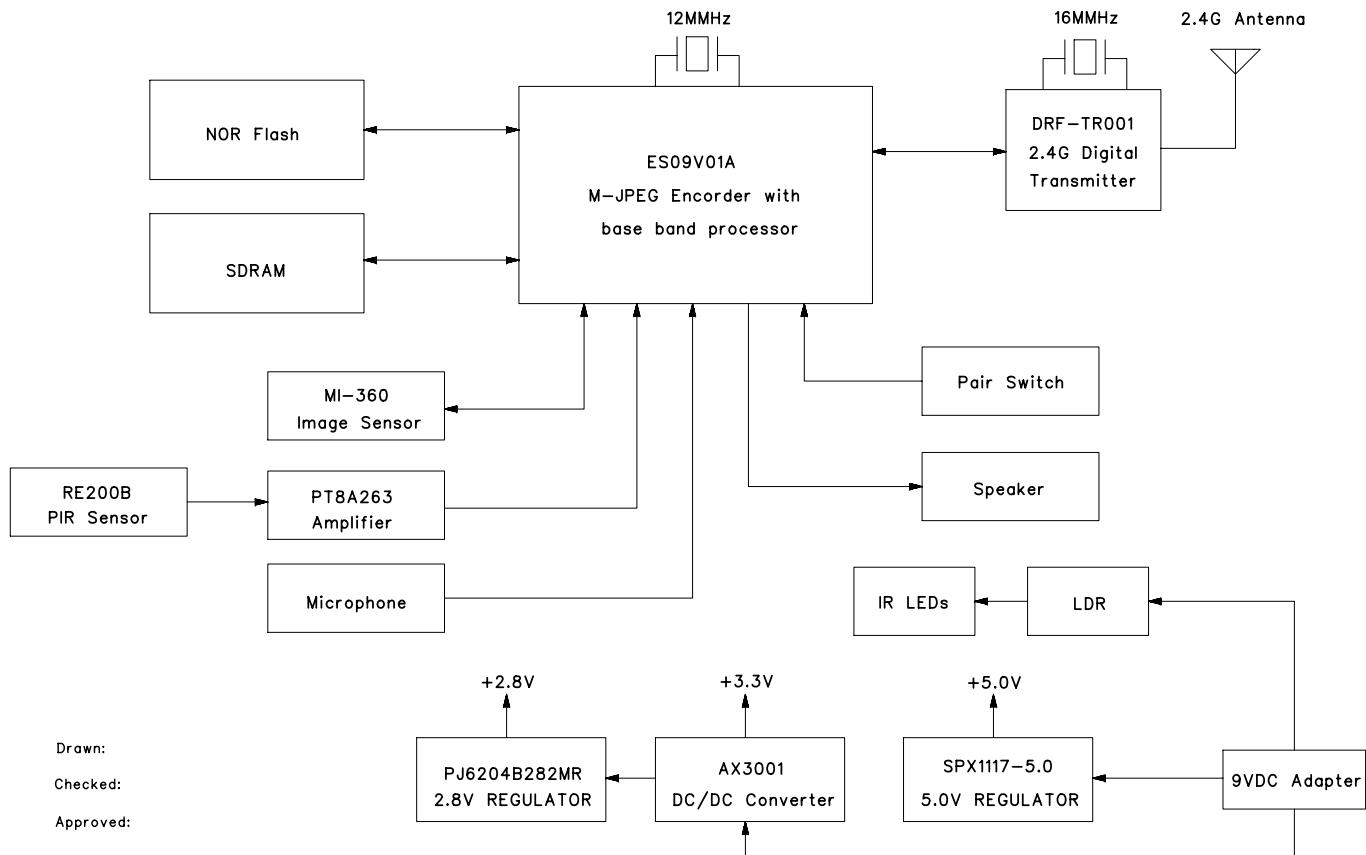
Figure 1: CA630 SR Block Diagram
