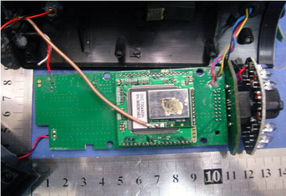
PCB1 - Front View
