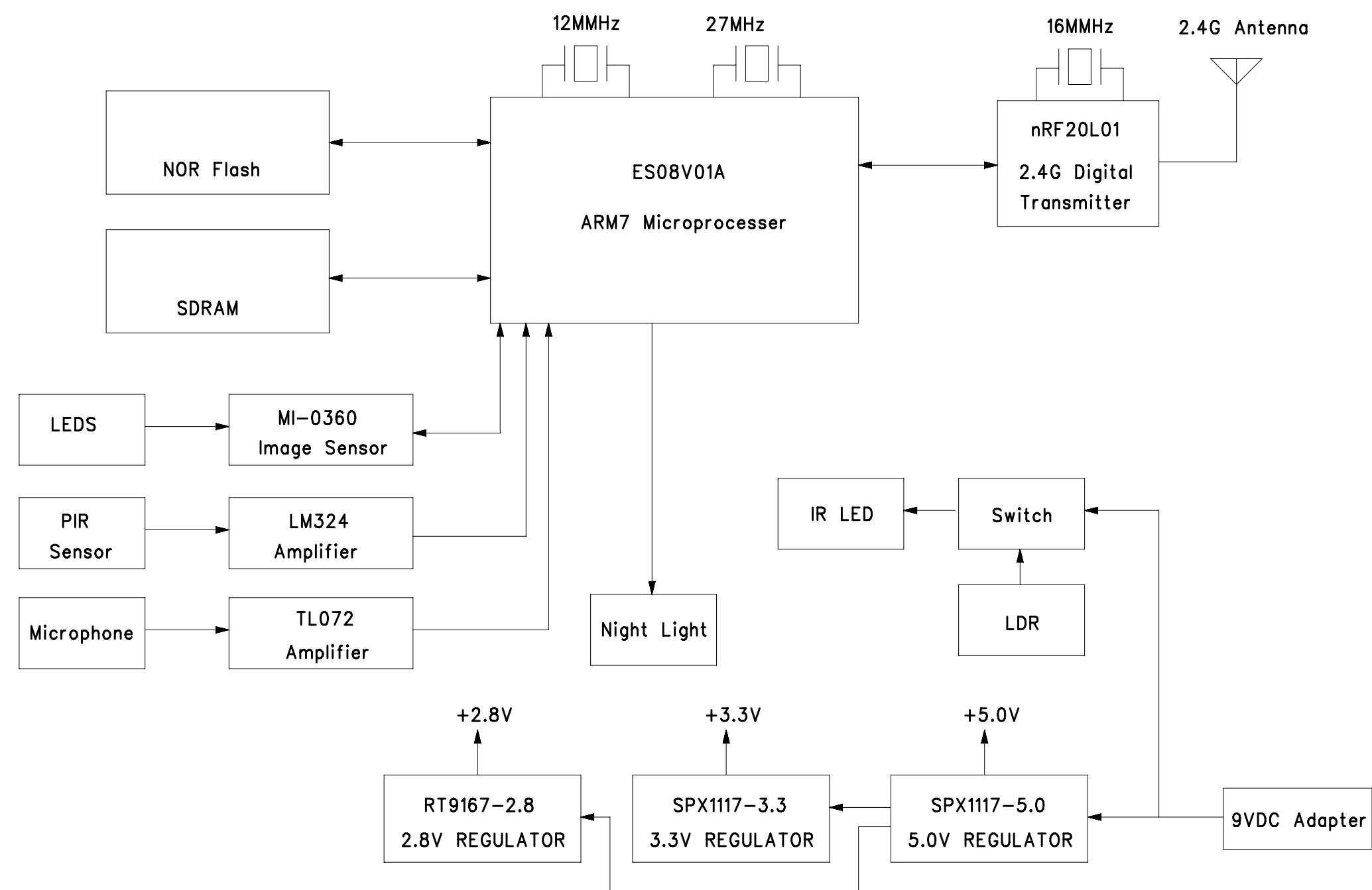
Figure 1: CA610 Block Diagram
