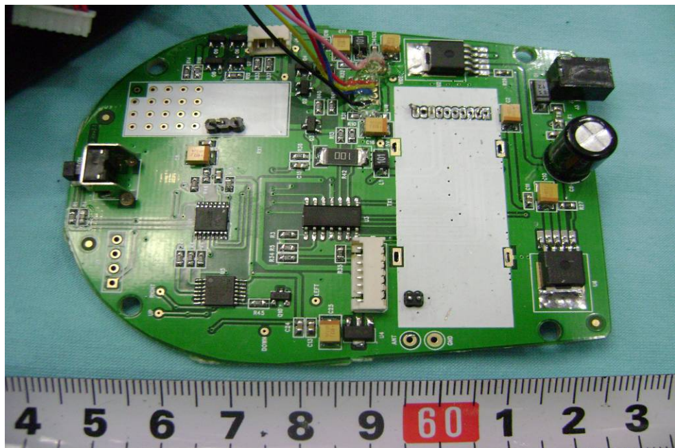
PCB5 - Back View
