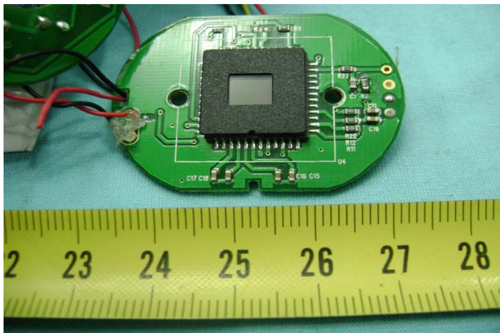
PCB4 - Back View
