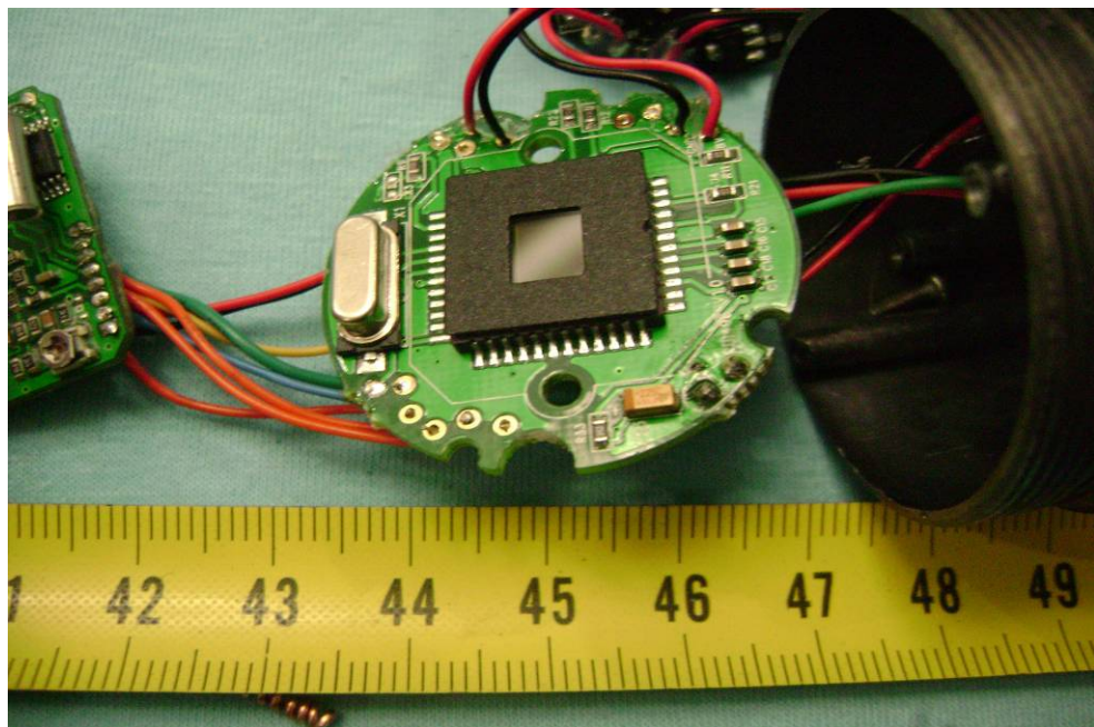
PCB2 - Front View
