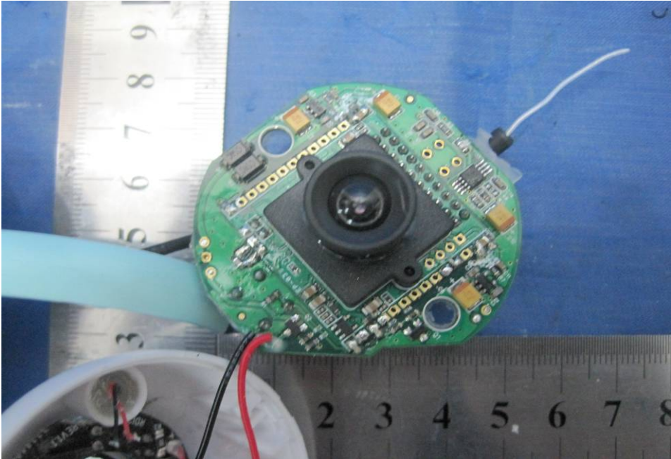
2.2PCB1 - Back View
