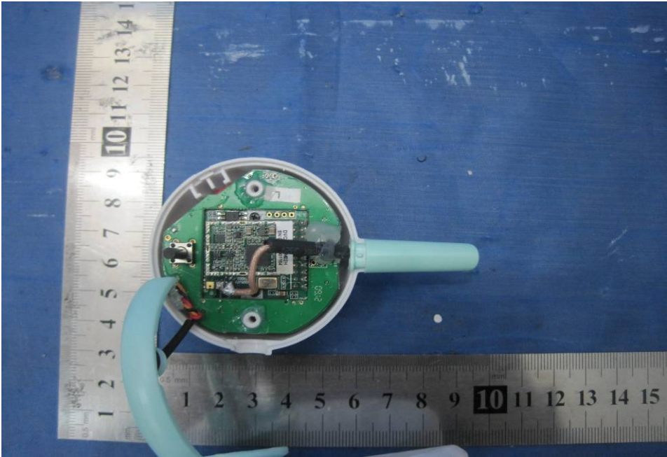
2.1PCB1 - Front View
