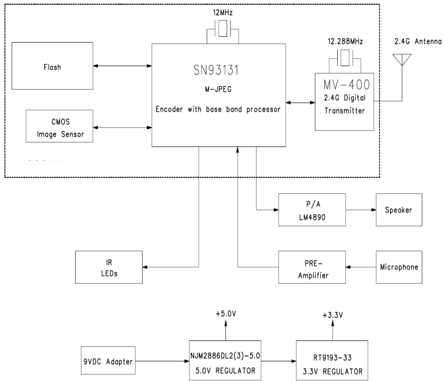
Figure 1: CA200L Block Diagram
