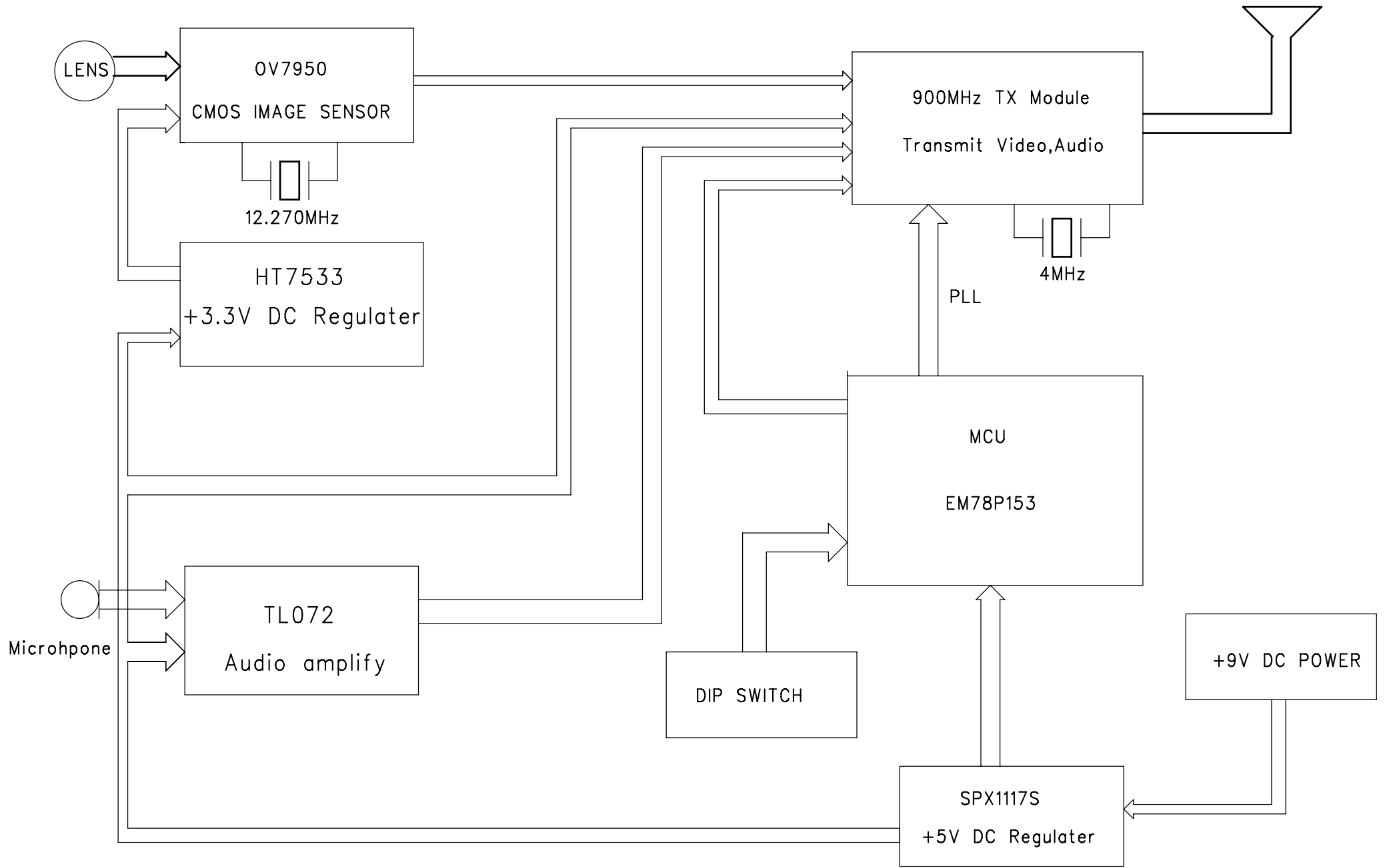
Figure 1. CA190 Block Diagram
