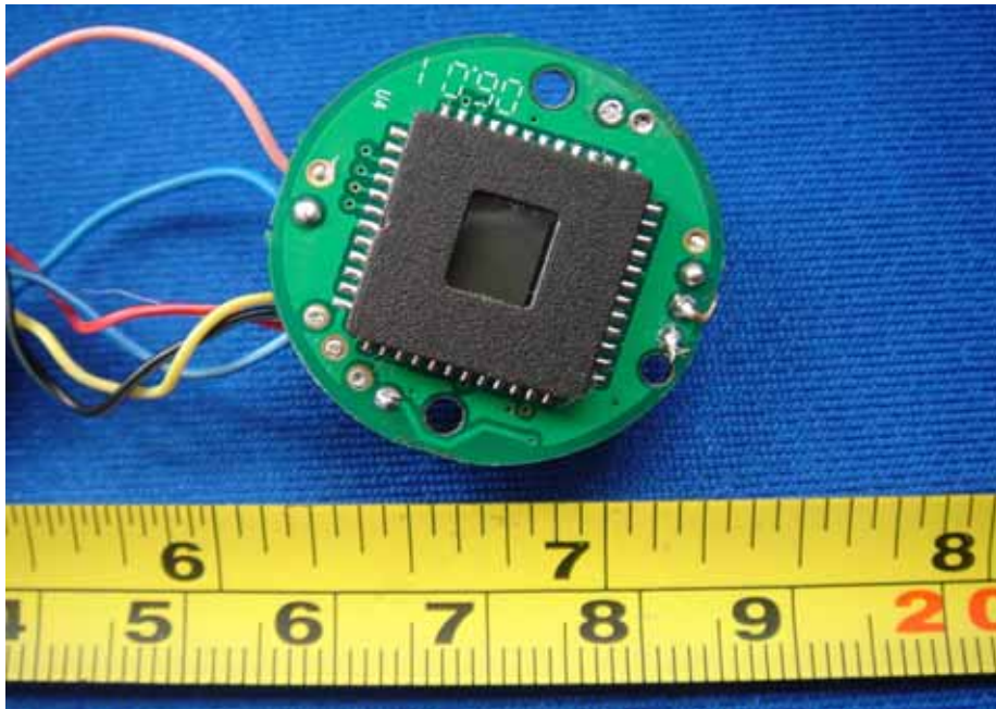
PCB 3- Component View
