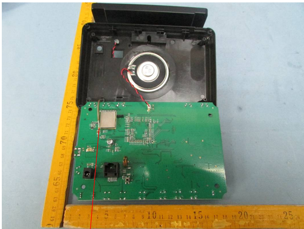
ANT. connector
