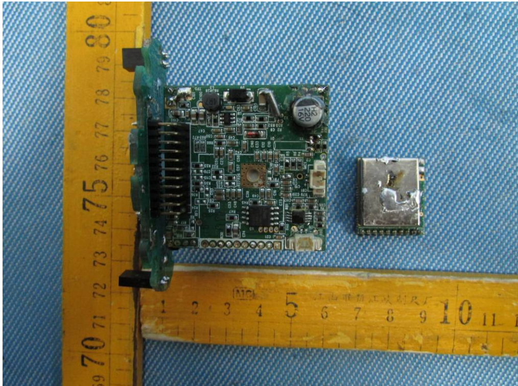
RF ANT.
