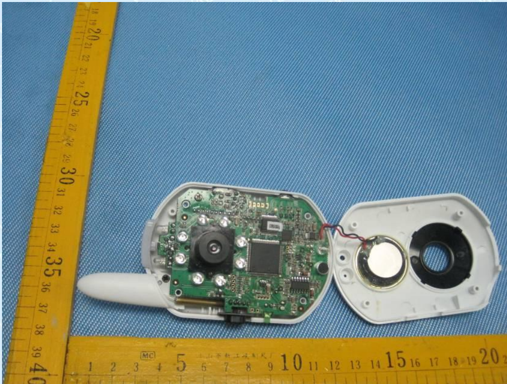
17.4 EUT - PCB View
