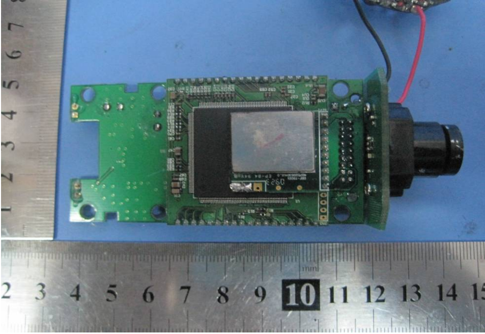
2.2PCB1 - Back View
